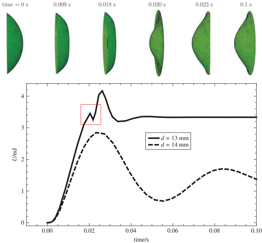
Figure 3. Strain energy plots for FE simulations of a symmetrically supported shell (bottom). A series of simulations were performed at different distances to mark the location of the transition location – shown here to be between 13 and 14 mm. The successful transitions display a snap-through event and an energy minimum marked on the plots with a red square. The FE simulations afford us a closer look at the intermediate geometries (top). For the idealized symmetric case, the transition shapes are axisymmetric, an effect that we were unable to capture in a physical setup. Shown here is the spherical cap, with its center at a distance of 13 mm from the center of the magnet we describe in the text. The magnetic poles are along the z -direction.
