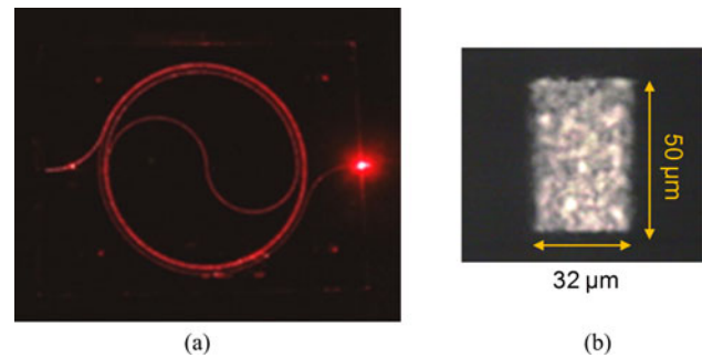
Fig. 1. Images of (a) the 1 m long spiral waveguide illuminated with red light and (b) the waveguide output facet illuminated with 850 nm light.
