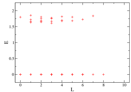
FIG. 3. Spectrum of the two-body contact interaction in the \uparrow\downarrow basis, \hat{\mathcal{H}}_{220}^{\uparrow\downarrow} , for N = 8 particles on a sphere with N_\phi = 8 flux quanta, i.e., n = 2 flux quanta above the ground state. The Hamiltonian has a large number of zero-energy states, but the degeneracy of this quasihole subspace is found to be lower than the corresponding degeneracy obtained for the case of \hat{\mathcal{H}}_{3-2} . The system features a large gap of \Delta \simeq 1.609 (known to be robust in the thermodynamic limit).
