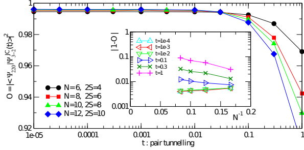
FIG. 1. Overlaps \mathcal{O} = |\langle \Psi_{220}^{\uparrow\downarrow} | \Psi_{3-2}^{JC}(t) \rangle|^2 between ground states of the three-body Hamiltonian with Josephson coupling (5) and the 220 state in the \uparrow\downarrow basis, the ground state of (12). Data is shown for systems with N = 6, \dots, 12 particles on the Haldane sphere. Inset: scaling of the difference |1 - \mathcal{O}| with system size, highlighting the change in behaviour: the overlap decreases with N in systems with t \gtrsim 0.03 , while it increases for t \lesssim 0.03 .
