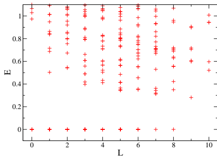
FIG. 2. Spectrum of the model Hamiltonian (1) for N_\uparrow + N_\downarrow = 4 + 4 on a sphere with N_\phi = 8 flux quanta, i.e., n = 2 flux quanta above the ground state as a function of total angular momentum L . The counting of quasihole states in the zero-energy manifold matches the theoretical prediction given in Eq. (18). We further identify the gap in this finite-size system to be \Delta_{N=8} \simeq 0.2812 .
