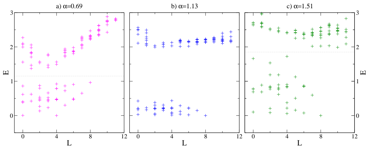
FIG. 4. Spectrum of the generalized pair tunneling Hamiltonian (13) for N = N_\uparrow + N_\downarrow = 8 on a sphere with N_\phi = 8 flux quanta, i.e., n = 2 flux quanta above the ground state as a function of total angular momentum L . Energies are given in natural units of V_0 , relative to the lowest energy state at each \alpha . Spectra are shown for a) \alpha = 0.22\pi \simeq 0.69 , b) \alpha = 0.36\pi \simeq 1.13 , and c) \alpha = 0.48\pi \simeq 1.51 . For values \alpha \simeq 1 , such as shown in panel b), there is a clear gap. Tuning further away from \alpha = 1 , the quasihole spectrum acquires more dispersion, and finally merges into the continuum of excited states. Panels a) and c) show spectra near the lower and upper boundary of the region in \alpha for which the counting of quasihole states in the low-energy manifold still matches the count of states for \hat{\mathcal{H}}_{220} . Grey dashed lines highlight the separation of the low-energy manifold of states and other excited states.
