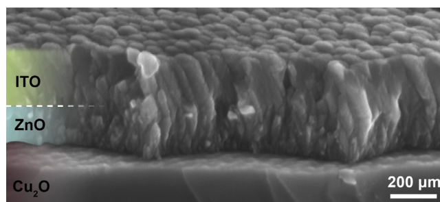
Fig. 2. Cross-sectional SEM image of ITO/ZnO/Cu 2 O heterojunction.
