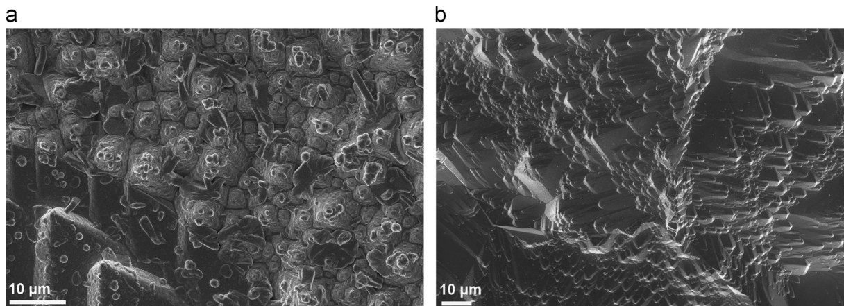
Fig. 5. SEM images of the top surface of \text{ZnO}/\text{Cu}_2\text{O} solar cells formed using (a) standard conditions and (b) optimized conditions of ZnO AALD deposition. Multiple whisker-, rod- and flower-like formations are present in the standard device.
