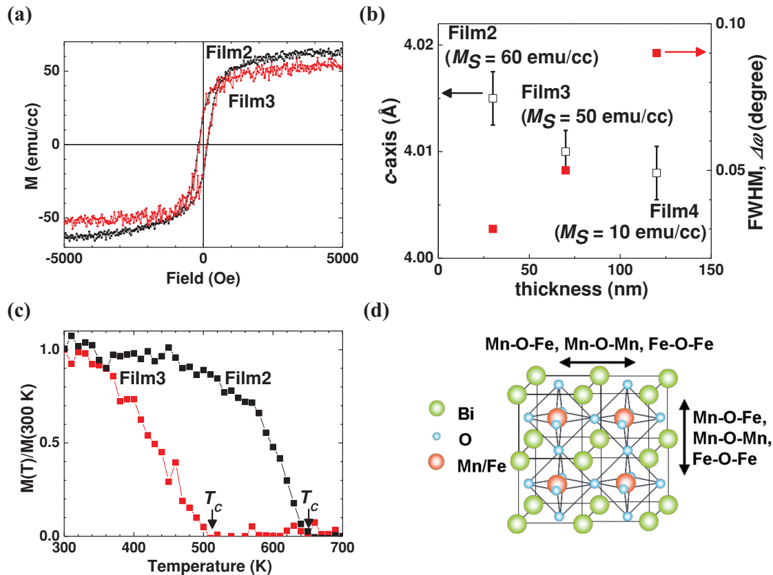
Figure 2. Strain effect on the magnetic properties of BFO films: a) Magnetic hysteresis ( M-H ) curves in the range of -5 \leq H \leq 5 kOe at RT with the field applied in the sample plane for Film2 (black square) and Film3 (red square). b) The relationship between c -axis lattice parameter (open squares), FWHM of \omega -rocking curves (red squares) and film thickness. c) Normalized in-plane M-T curves of Film2 and Film3. The magnetic transition temperatures of Film2 and Film3 are > 600 K and \sim 500 K, respectively. d) Schematic illustration for disordered \text{BiFe}_{0.5}\text{Mn}_{0.5}\text{O}_3 structure and various combinations of B-O-B' bond.
