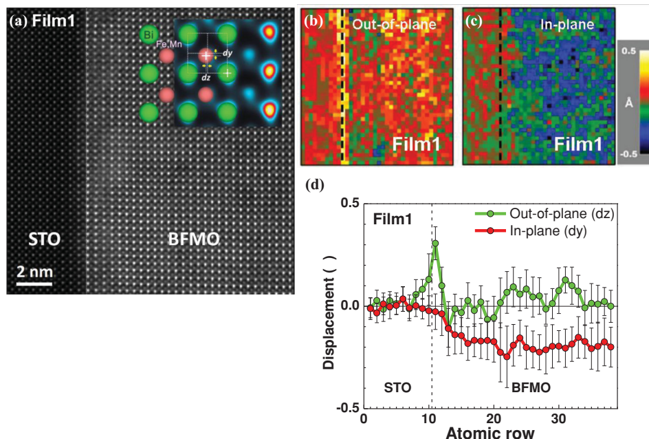
Figure 6. Polarization mapping by atom position quantification: a) Atomic resolution ADF STEM image of [100] oriented BFMO film on STO sample analyzed for polarization behavior. Inset: enlarged ADF STEM image in false color and atomic model to illustrate atom position quantification. b,c) Out-of-plane ( dz ) and in-plane ( dy ) displacement maps of B-site cations in BFMO thin film. d) Line profiles averaged over vertical rows of the maps (b – green and c–red). Dotted lines in each figure indicate the position of the interface between BFMO and STO substrate.
