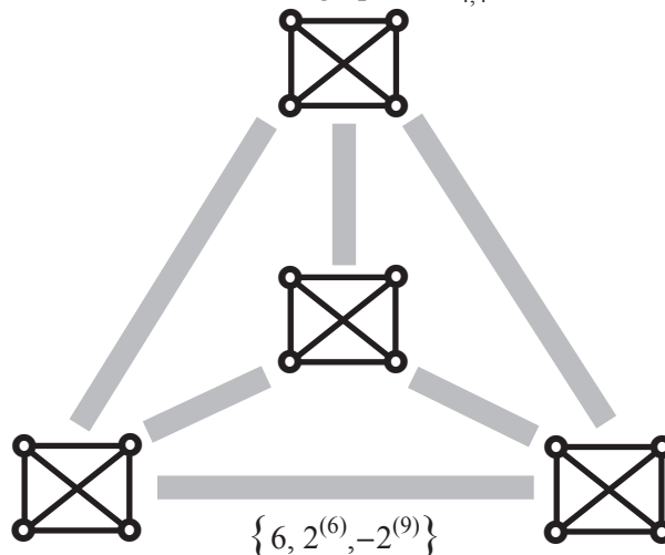
The line graph of K_{4,4}
