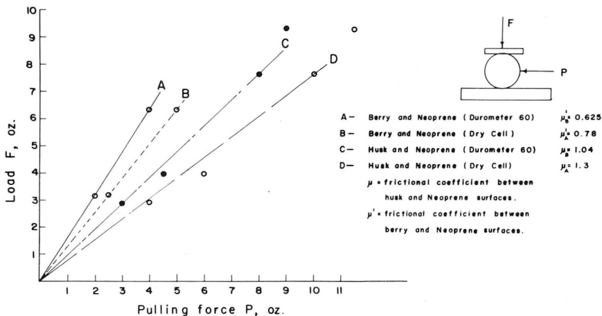
FIGURE 3. Frictional coefficients between poha berry, husk, and two rubber surfaces.
