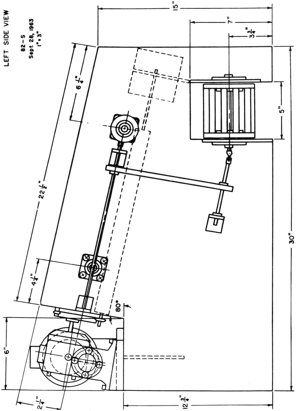
FIG. A-2. Dimensional drawing of mechanical polka berry husker. Side view.
