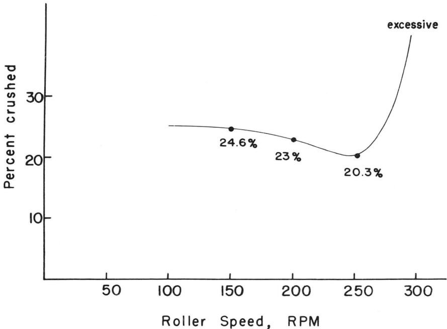
FIGURE 5. Effect of roller speed on crushing percentage.
