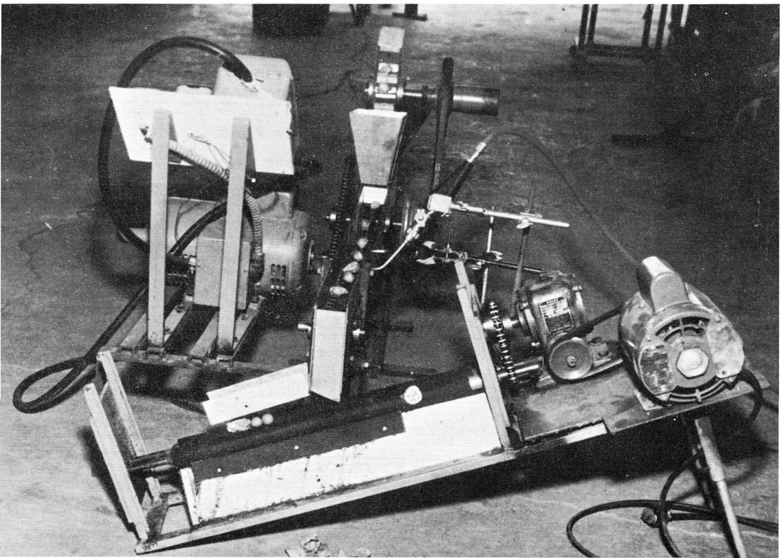
FIGURE 7. Laboratory husker.
