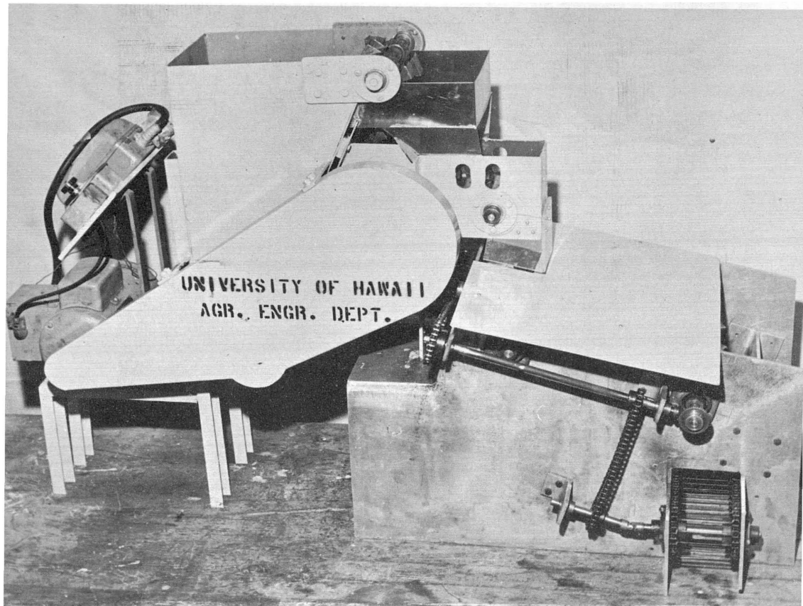
FIGURE 9. Side view of the laboratory husker.
