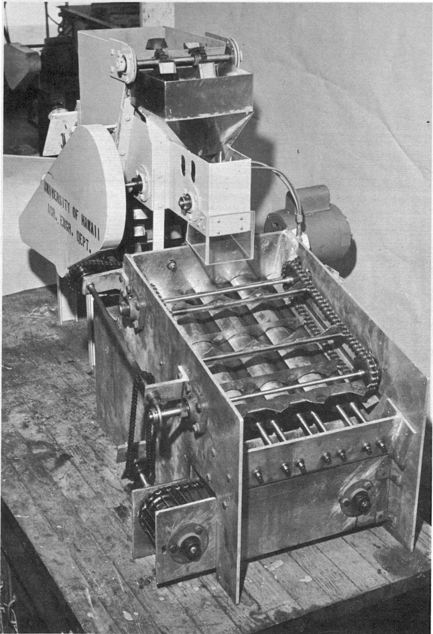
FIGURE 8. Laboratory husker with a feeder and a precutting attachment.
