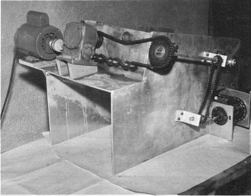
FIGURE 10. Prototype husker and its drive mechanism.
