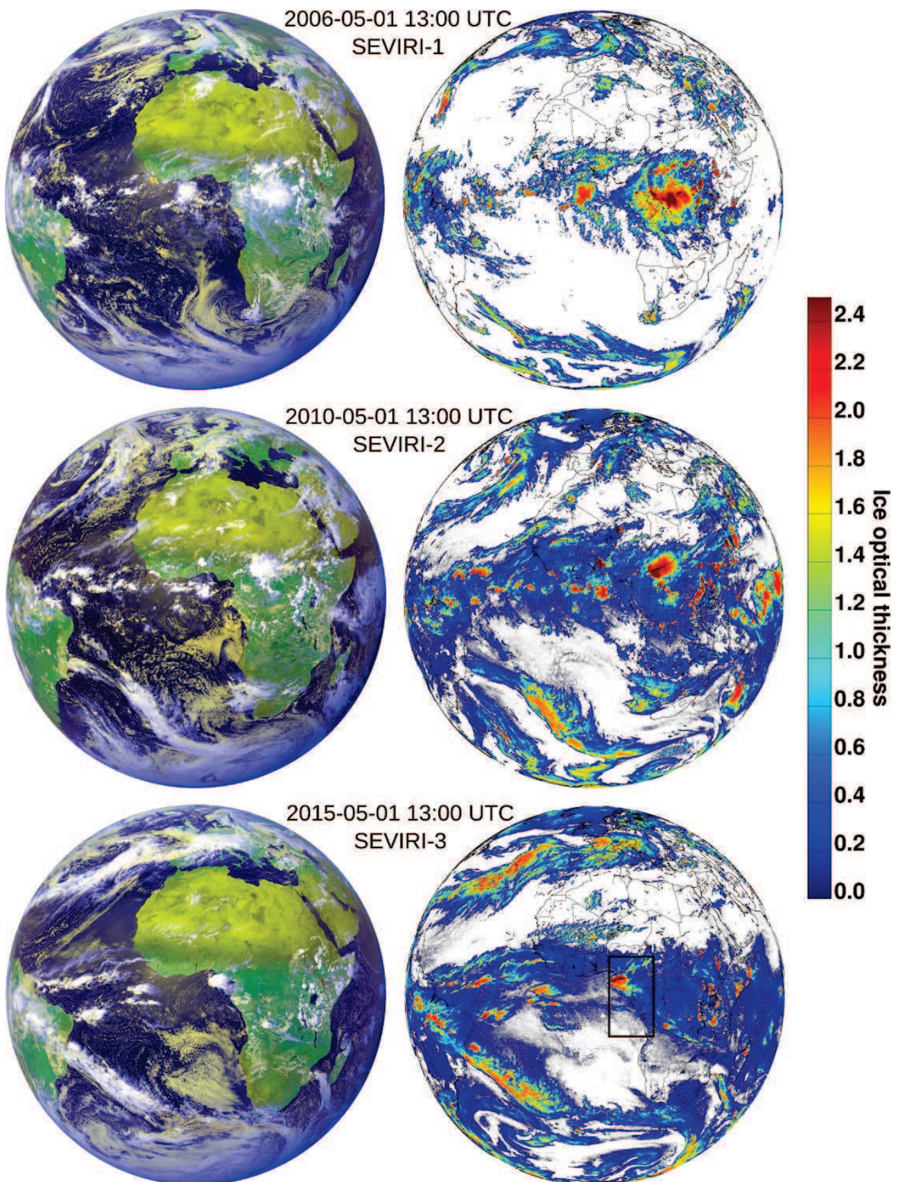
Figure 1: SEVIRI false color RGB composites (left column) and ice optical thickness retrieved by COCS (right column) using SEVIRI-1 (top), SEVIRI-2 (center) and SEVIRI-3 (bottom). Ice clouds are recognized as white or bluish in the false color composites, whereas liquid water clouds are recognized as yellowish. The black rectangle in the bottom right figure shows the region studied in more detail in section 2.2
