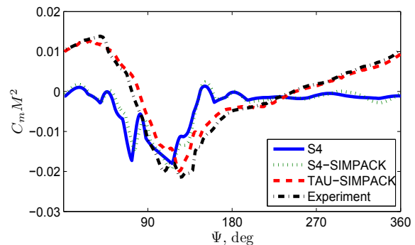
FIG 10 Section moment coefficient at r/R=0.98
