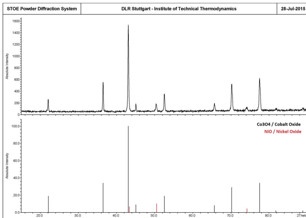
Figure 11: XRD of CoNi foam
