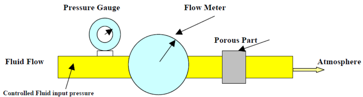
Figure 2: Systematics of permeation test
