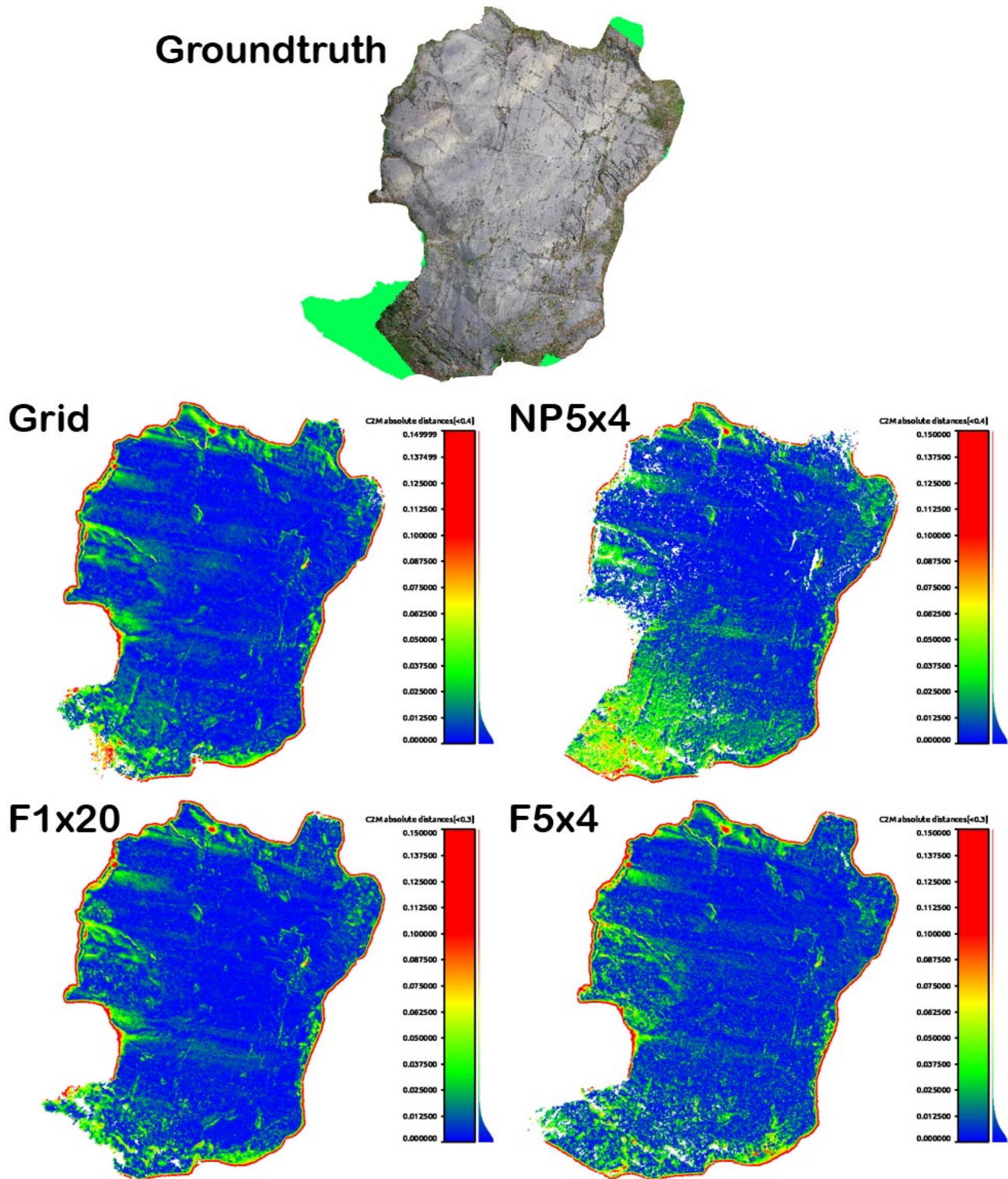
Figure 13. Distance to the groundtruth. On the top we show the groundtruth mesh which has been acquired with terrestrial laser scanning and was partly textured with UAV acquired images. The other images show the color coded distance of the final reconstructions to the groundtruth mesh. Note that the error of Grid, F1x20 and F5x4 is very similar, while NP5x4 has a much larger error in the bottom part of the rock. Further notice that F5x4 has the largest coverage of the rock surface in the lower left corner of the rock.
