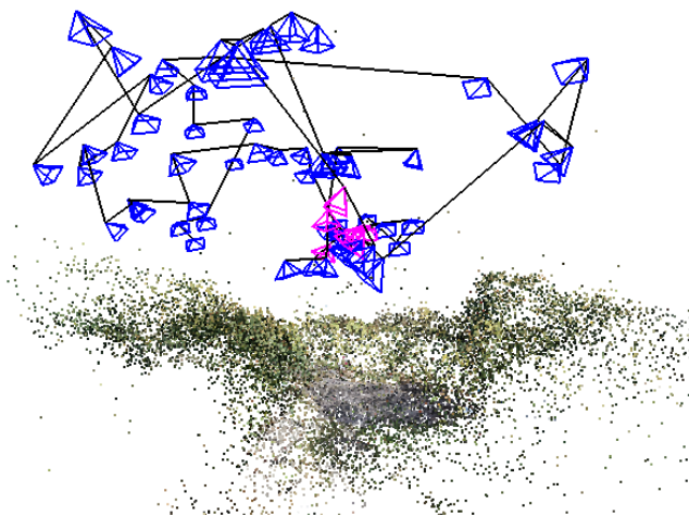
Figure 10. View plans of our approach without structure updates (F1x20). In this version the approach only planned a single view plan. We show the view plan together with all 3D points that were generated on-site during the acquisition. The blue cameras belong to the planned camera triplets, whereas the pink cameras ensure a successful registration during the acquisition.
