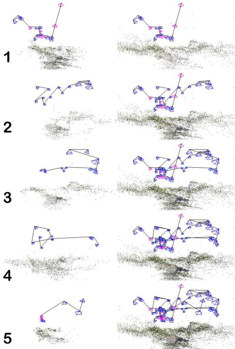
Figure 8. View plans of our full approach (F5x4). From top to bottom we show the five planning iterations. On the left side, we show the current view plan together with the 3D points that were added to the sparse reconstruction with these images during the acquisition. On the right side, we show the sparse reconstruction at the time of planning and all computed view plans up to this point. The blue cameras belong to the planned camera triplets, whereas the pink cameras ensure a successful registration during the acquisition.
