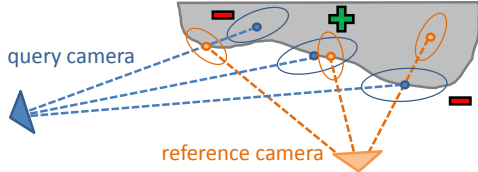
Figure 2. Consistency voting. A positive vote (center) is only cast if the reference measurement is within the uncertainty boundary of the query measurement. A negative vote is either cast if a reference measurement blocks the line of sight of the query camera (left) or the other way around (right).
