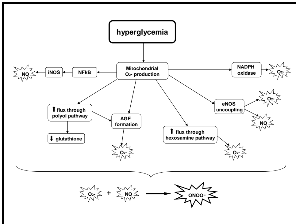
Figure 1.9 Mechanisms by which hyperglycemia increases peroxynitrite formation. Abbreviations: O_2^- , superoxide anion; NFκB, nuclear factor κB; iNOS, inducible nitric oxide synthase; NO, nitric oxide; NADPH oxidase, nicotinamide adenine dinucleotide phosphate oxidase; AGE, advanced glycation end-product; ONOO - , peroxynitrite.
