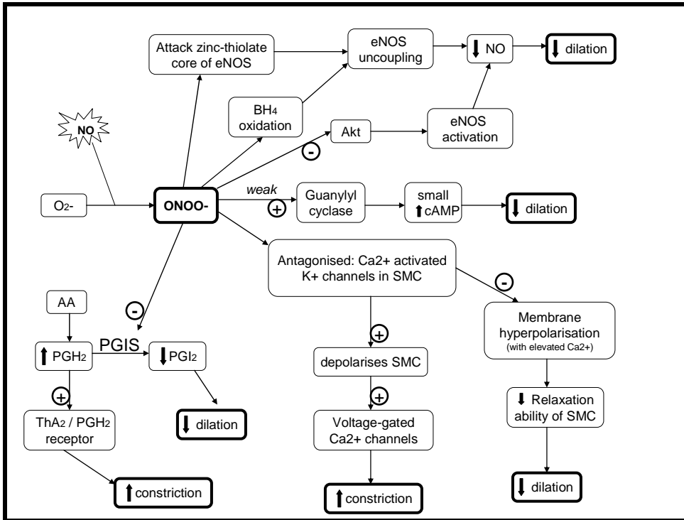
Figure 1.8 The effect of peroxynitrite (ONOO - ) on mechanisms controlling vasodilation and vasoconstriction. Abbreviations: eNOS, endothelial nitric oxide synthase; NO, nitric oxide; O 2 - , superoxide anion; AA, arachidonic acid; PGH 2 , prostaglandin H 2 ; PGIS, prostaglandin I 2 synthase; PGI 2 , prostaglandin I 2 ; ThA 2 , thromboxane A 2 ; BH 4 , tetrahydrobiopterin; cAMP, cyclic adenosine monophosphate; Ca 2+ , calcium ion; K + , potassium ion; SMC, smooth muscle cell.
