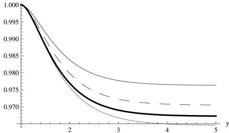
Figure 1: Hitting probabilities \mathbb{P}_x^y(\tau_y^+ < \tau_0^-) as a function of y \geq x = 1 (in bold) and some hypotheses.
