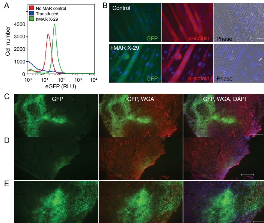
Figure 3: In vitro and in vivo differentiation of clonal eGFP-expressing mesoangioblasts.
