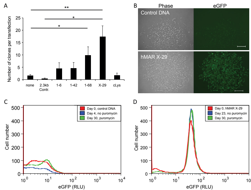
Figure 2: Effect of MARs on mesoangioblast stable transfection efficacy.
