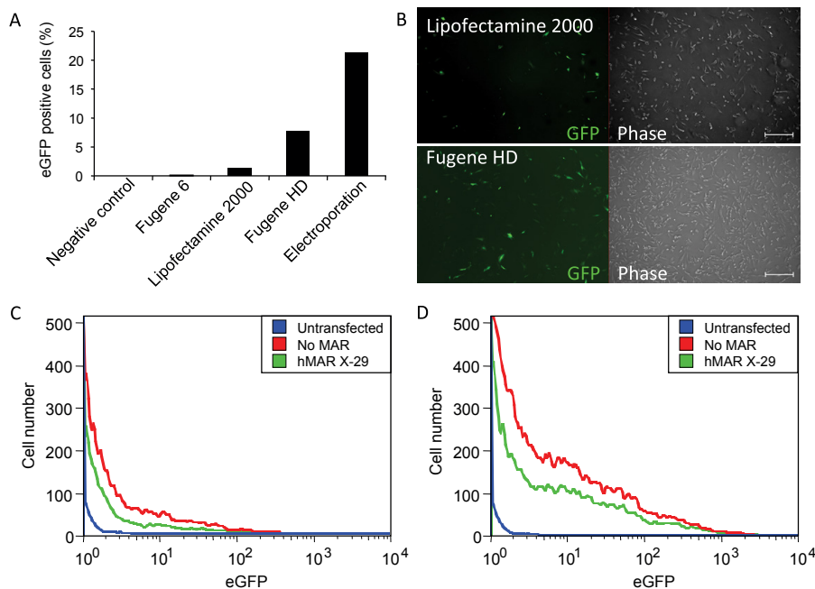
Figure 1: Transfection of primary murine mesoangioblasts by various approaches. Transfection was done according to manufacturer's instructions using optimized amounts of DNA. The percentage of eGFP positive cells was recorded 48 h after transfection by FACS cytofluorometry (A) or fluorescence microscopy (representative fields shown, panel B). Scale bars indicate 200 \mu m. FACS profiles of eGFP expression obtained from the hMAR X-29-containing vector of from a control construct devoid of any insert (no MAR), as determined 48 h after transfection with lipofectamine 2000 (C) or Fugene HD (D) Cells were transfected with equimolar amounts of either the no MAR eGFP or the hMAR X-29 eGFP plasmid.
