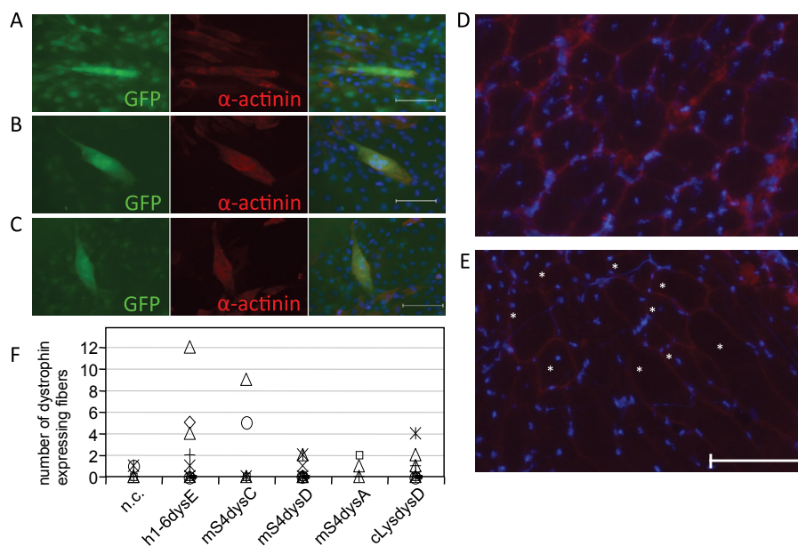
Figure 5: Differentiation and in vivo dystrophin expression from transfected mesoangioblast stable cell clones. In vitro differentiation assays were performed on all selected clones, and the eGFP expression, \alpha -actinin staining and an overlay are shown at day 7 after a co-culture with C2C12 cells in the co-differentiation assay conditions. A representative clone for each of the expression construct is shown, namely clone h1-6dys.E (panel A), cLysdys.D (panel B) and mS4dys.C (panel C). Scale bars represent 100 \mu m. (D) Dystrophin staining on cross-section of TA from a 5 wk old C57Bl6 mouse (positive control, panel D) and cross-section of a TA from a 5 wk old mdx mouse 1 month after a single intra-muscular injection with 5 \times 10^5 cells of the S4dys.D clone (panel E). Mdx mice were immunosuppressed by daily injections of FK506 before sacrifice, and dystrophin-positive fibers were counted in distal and proximal transversal sections of each TA muscle. The scale bar represents 50 \mu m. (F) Dystrophin positive fibers were counted for the negative control (n=6) and after transplantation of cells from the h1-6dys.E (n=12), mS4dys.C (n=6), mS4dys.D (n=12), mS4dys.A (n=4), or cLysdys.D (n=10) clones.
