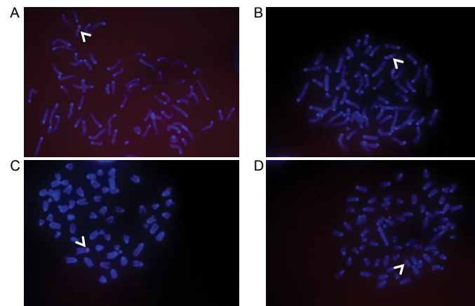
Figure 4: Clones derived from plasmid transfection have single genomic integration sites. Representative FISH images of clones used for in vivo transplantation studies. Arrows indicate the transfected plasmid integration sites. Inlays are enlargements of transgene-bearing chromosomes. (A) eGFP clone X29.J. (B) eGFP clone noMAR.B. (C) eGFP clone S4.B. (D) eGFP clone 1-6.E.
