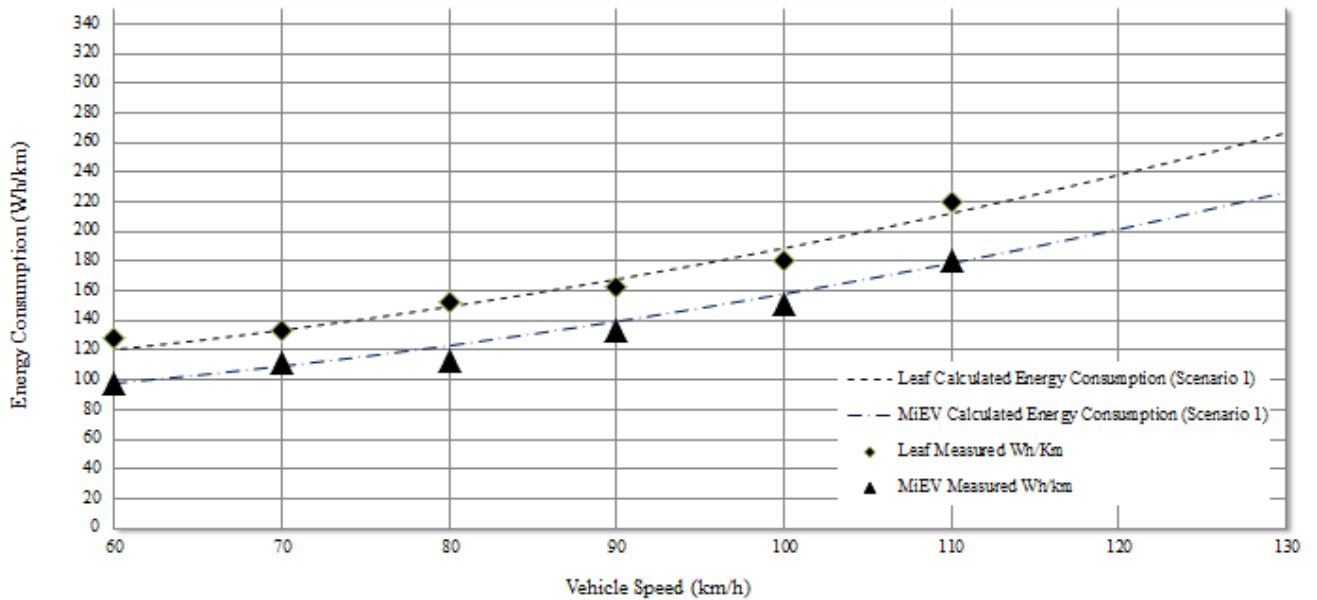
Figure 2: Measured and extrapolated energy consumption over a speed range of 60 to 130 km/h.
