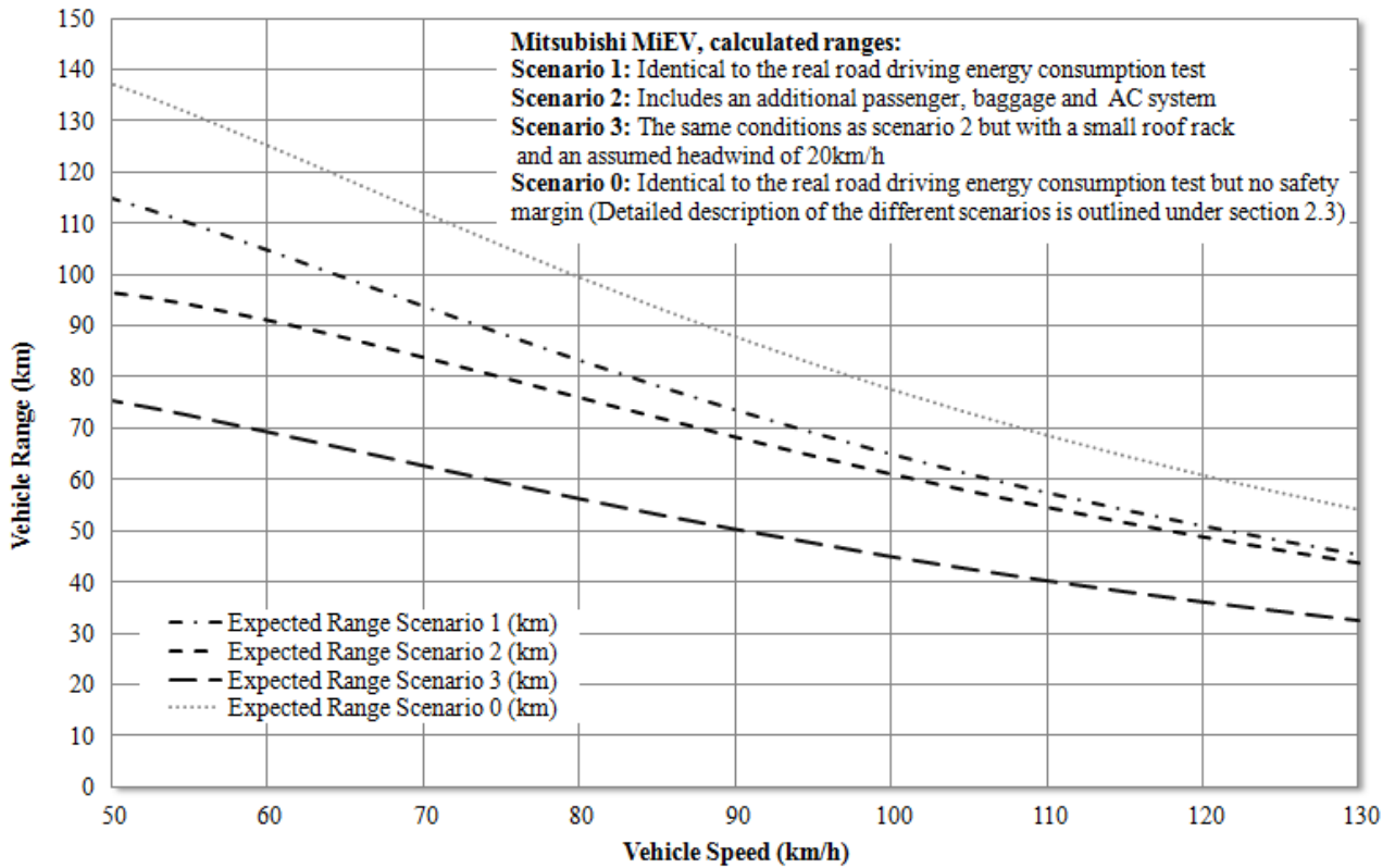
Figure 3: Leaf (A) and MiEV's (B) significant decline in drivable range due to an assumed battery discharge safety margin of 2 kWh, increased speed, mass and loads
