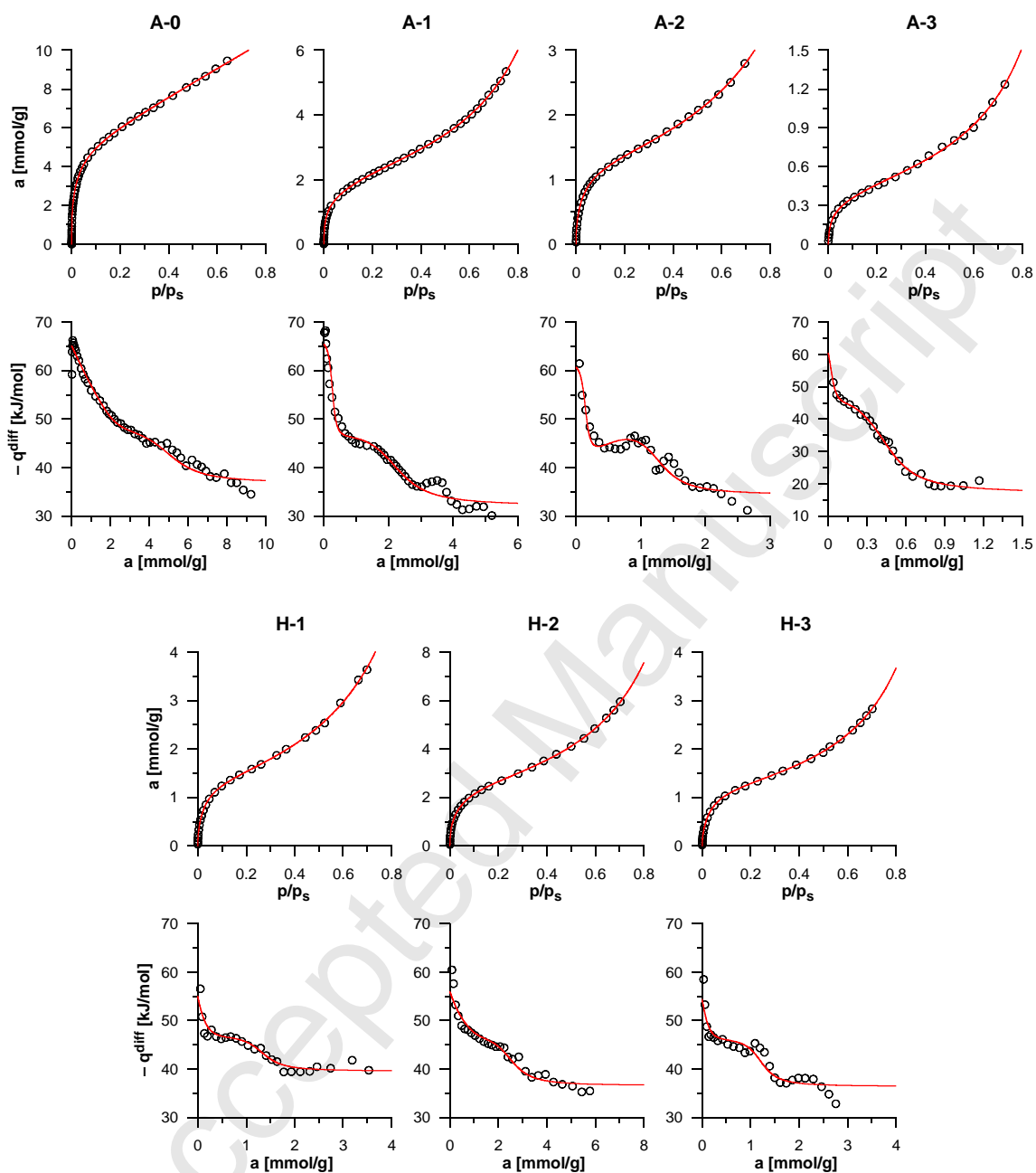
Figure 2. Graphical representation of the experimental data ( C_6H_6 adsorption isotherms and related enthalpy) fitting by the MSGDW model (Eqs (1) and (5)). Points - experimental data, lines - theoretical model.
