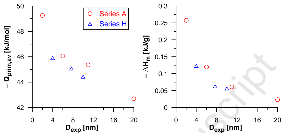
Figure 3. The correlation between average energy of adsorption on primary sites ( Q_{prim,av} , Eq. (12)) or the total energy of interaction of molecules binding in monolayer ( \Delta H_m , Eq. (13)) and the diameter of nanotubes.
