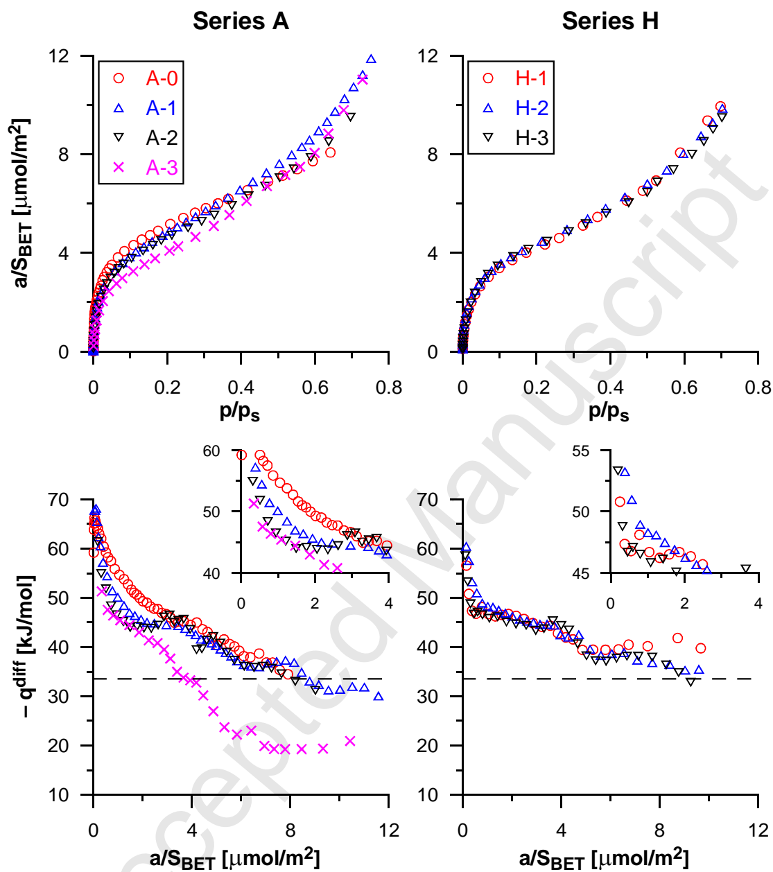
Figure 1. The comparison of benzene adsorption isotherms ( T = 298 K) and related differential enthalpy of adsorption for all the considered nanotubes. The dashed lines on lower panels represent the enthalpy of benzene condensation.
