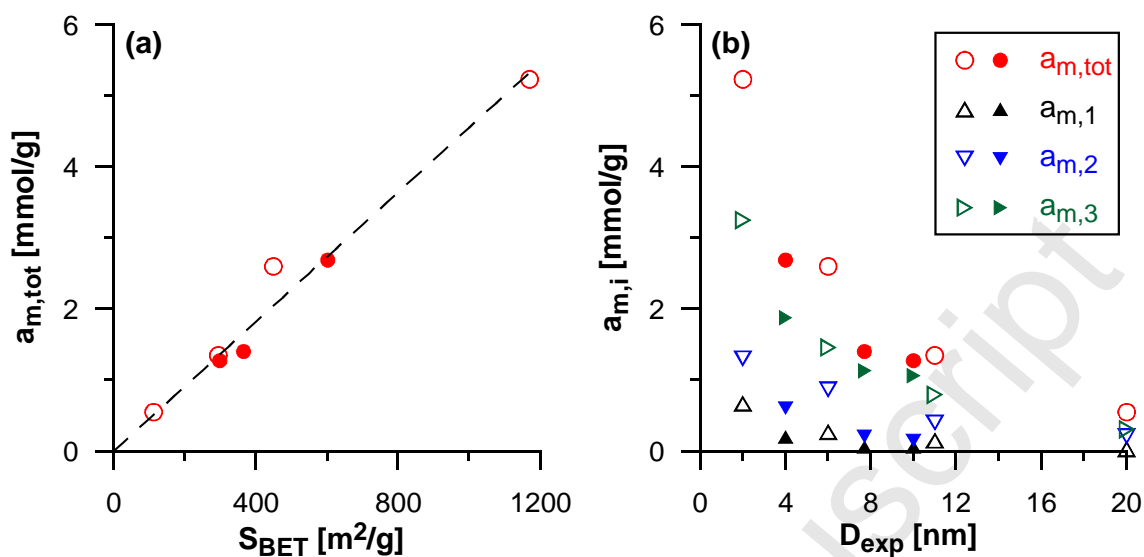
Figure 4. (a) Correlation between total concentration of primary sites calculated from the MSGDW model ( a_{m,tot} = \sum_{i=1}^3 a_{m,i} ) and the BET surface area (open and full symbols are related to the A and H series, respectively; the dashed line is drawn to guide the eye). (b) The concentration of different kinds of primary sites (and their total concentration) plotted as the function of nanotube diameters.
