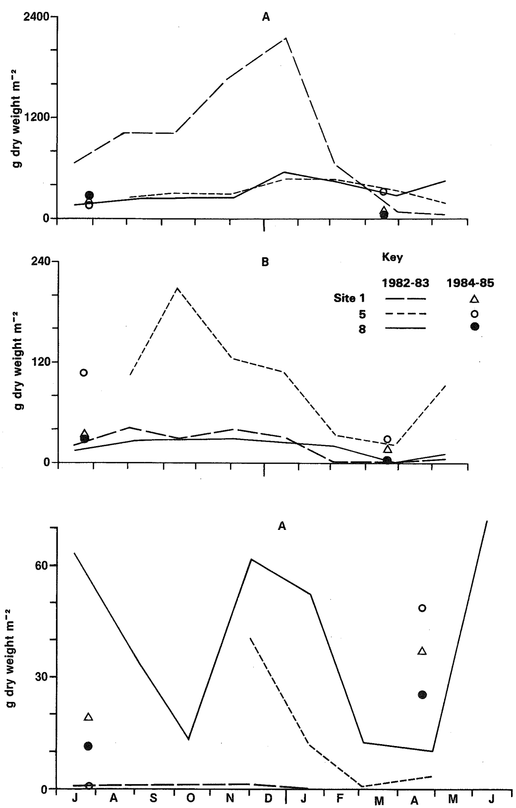
Figure 7. Seasonal changes in (A) Ruppia above-ground biomass; (B) Ruppia below-ground biomass; and (C) macrophyte biomass (excluding Ruppia ).
