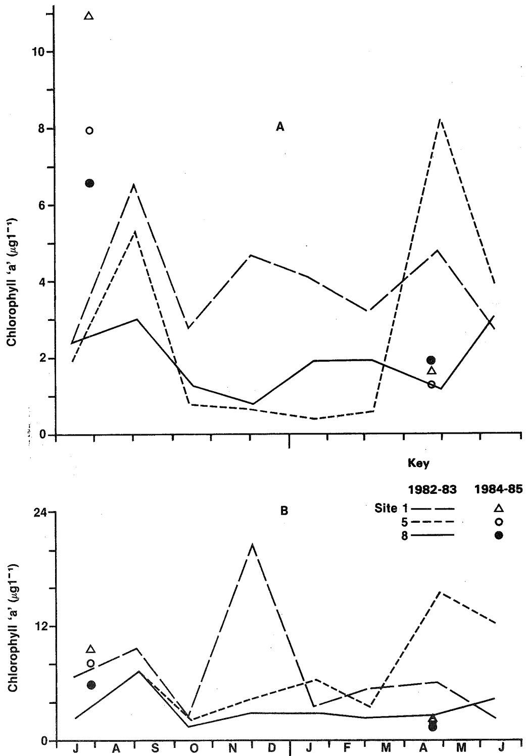
Figure 6. Seasonal variation in chlorophyll 'a' in Wilson Inlet. (A) surface; (B) mean concentration between a surface and bottom sample.
