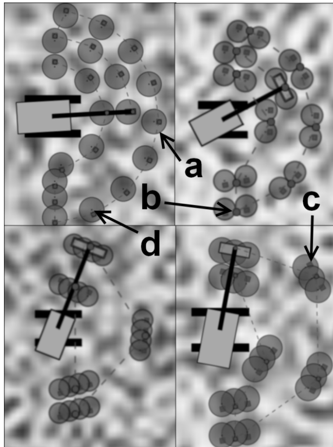
Figure 3. The ideal work patterns of the (clockwise from upper left) one-, two-, three-, and four-headed planting device models on humus-covered, obstacle-free terrain as depicted by the discrete-event simulation tool's visualization feature. The dashed lines illustrate the crane motion; the radius of the large, lightly shaded circles (a) is the minimum seedling spacing; the small darker circles (b) show each crane stop; the dark squares (c) illustrate the scoops; and the tiny dots close to the scoop (d) are successfully planted seedlings.
