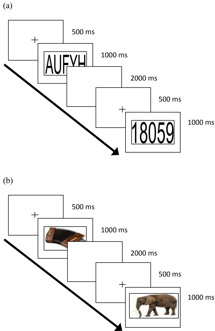
Figure 4. Schematic representations of the (a) Letter-Number visual task and (b) Animal-Musical instrument visual task.
