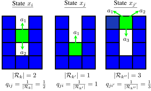
Fig. 3: Example of forward and reverse actions with their associated proposal probabilities q_{ij} , q_{ji} , and q_{ji}' . Note that x_i , x_j , x_j' are states of the entire configuration, and agent k is the currently active agent.
