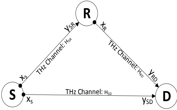
Fig. 1 System model of single relay assisted data transmission in the THz band at the nanoscale
