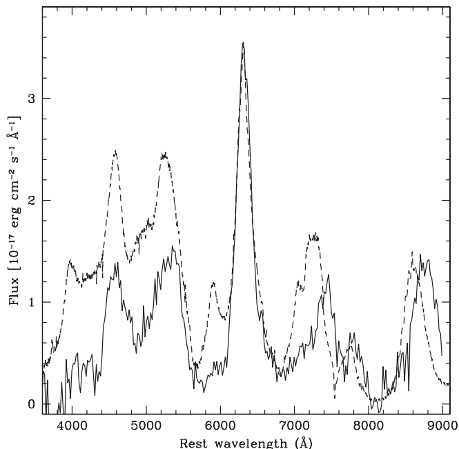
FIG. 2.—Spectrum of SN 2006aj obtained at the Keck Observatory on 2006 July 26, corresponding to a rest-frame epoch of 153 days after XRF 060218 (solid line), calibrated and binned with a 25 Å boxcar, compared to the spectrum of SN 1998bw spectrum obtained on 1998 September 12 (Patat et al. 2001), at an epoch of 139 days after the explosion, which is assumed to have occurred on 1998 April 25, in coincidence with the GRB (dashed line). The flux of SN 1998bw has been rescaled to match that of SN 2006aj at the peak of the [O I] line. [See the electronic edition of the Journal for a color version of this figure.]
