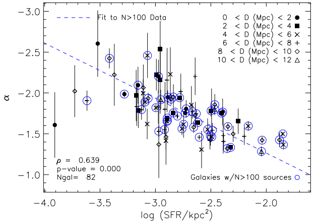
Figure 16. A plot of the LF slope ( \alpha ) versus \Sigma_{\text{SFR}} similar to that of Figure 10. We find a moderately strong trend between these two quantities. The blue-open circles represent galaxies with a total number of sources greater than 100 where we expect random scatter due to stochastic effects to be minimal. The correlation coefficient for galaxies with N > 100 is 0.705; stronger than that of all galaxies in the figure. The blue-dashed line is a bisector fit to the N > 100 data and is described by equation Eqn 7.
