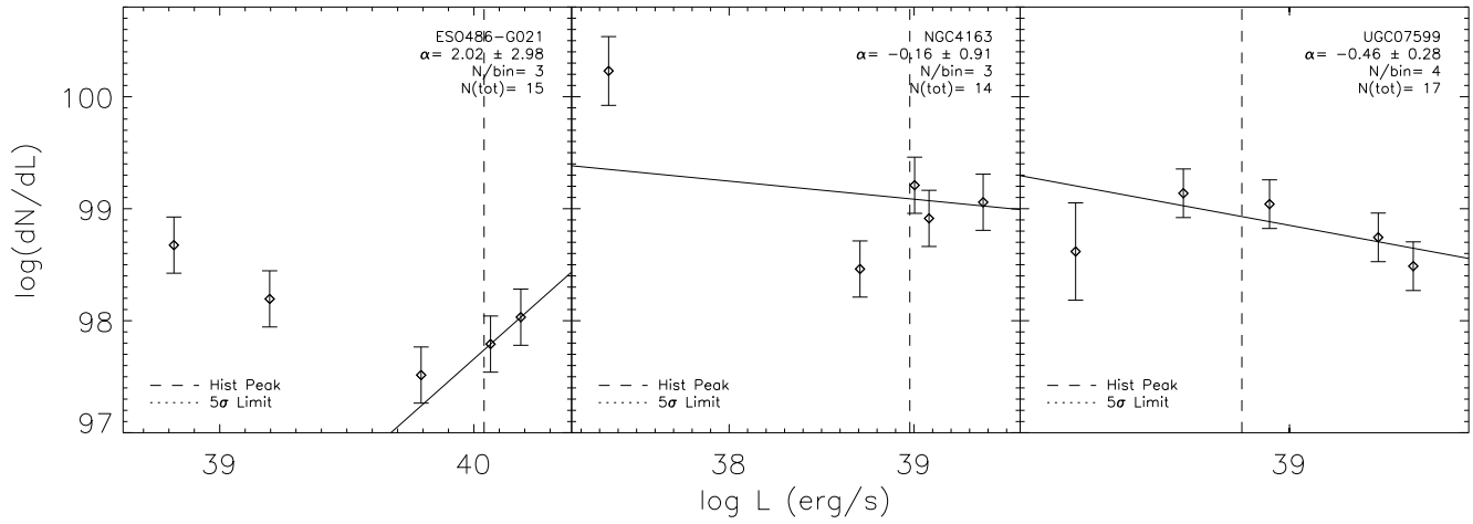
Figure 9. Examples of ill-behaved luminosity functions similar to the top panels of Figure 8. From left-to-right, these examples show LFs where: \log(dN/dL) values do not rise continuously towards fainter luminosity bins, the fit depends on only two or three data points, and the data are indistinguishable from a scatter plot. There are 11 galaxies whose LFs are similar to one or more of these examples. The y-axes have been normalized to an arbitrary number.
