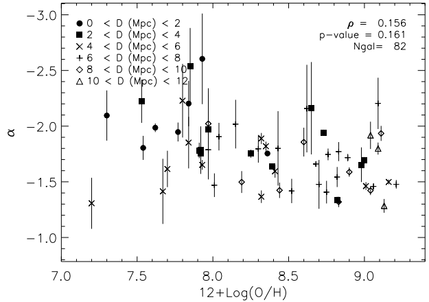
Figure 13. A plot of the LF slope ( \alpha ) versus metallicity similar to that of Figure 10. We find a no trend between these two quantities.
