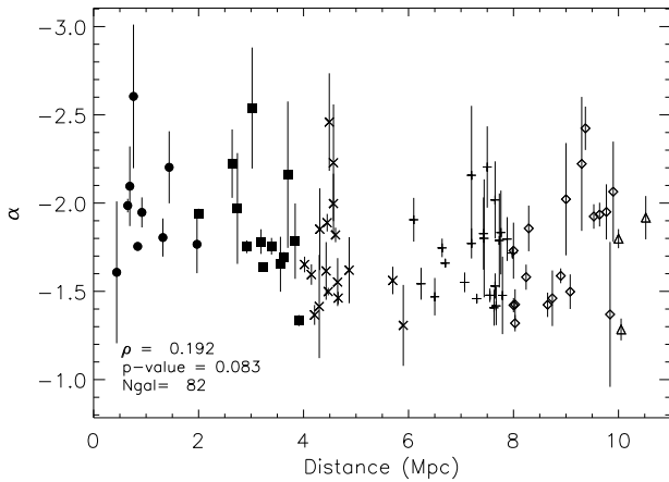
Figure 20. A plot of the LF slope ( \alpha ) versus distance similar to that of Figure 10. We find no trend between these two quantities indicating that resolution effects due to distance has little or no effect on our LF slope-galaxy property relationships.
