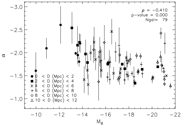
Figure 11. A plot of the LF slope ( \alpha ) versus absolute B -band magnitude ( M_B ) similar to that of Figure 10. We find a weak trend between these two quantities.
