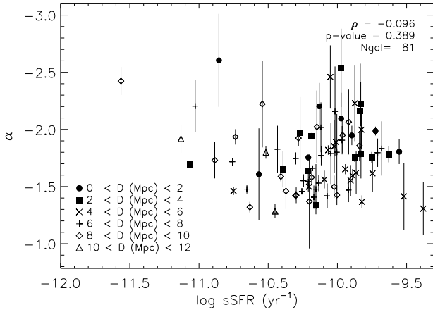
Figure 15. A plot of the LF slope ( \alpha ) versus sSFR similar to that of Figure 10. We find no trend between these two quantities.
