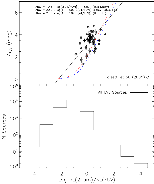
Figure 5. Top panel: the plot of extinction in the FUV bandpass ( A_{\text{FUV}} ) versus the logarithmic ratio of 24\mu\text{m}/\text{FUV} luminosities for the star-forming regions of Calzetti et al. (2005) in M51. The solid black line is the bisector fit to the data of Calzetti et al. (2005), the blue-dashed line is the relationship prescribed by Hao et al. (2011) for galaxies, and the red-dashed line is the relationship prescribed by Leroy et al. (2008); Liu et al. (2011) for individual regions. We use the relationship derived from the star-forming regions of Calzetti et al. (2005) to correct our FUV sources for flux attenuated by dust. Bottom panel: the histogram of the 24\mu\text{m}/\text{FUV} luminosity ratios for all identified star-forming regions in our study.
