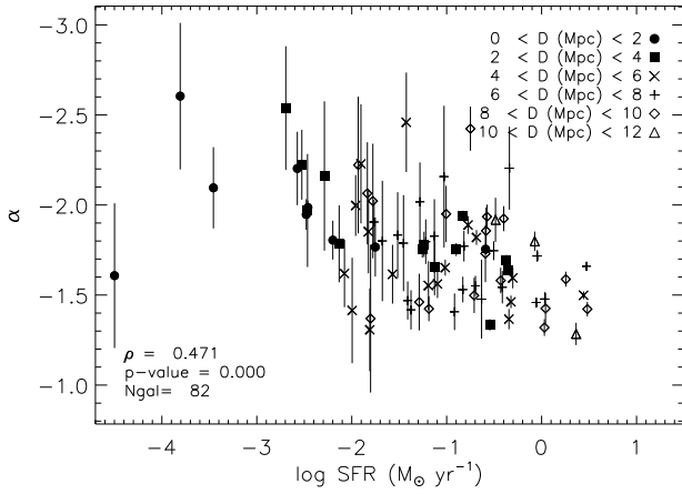
Figure 14. A plot of the LF slope ( \alpha ) versus SFR similar to that of Figure 10. We find a weak-to-moderately strong trend between these two quantities.
