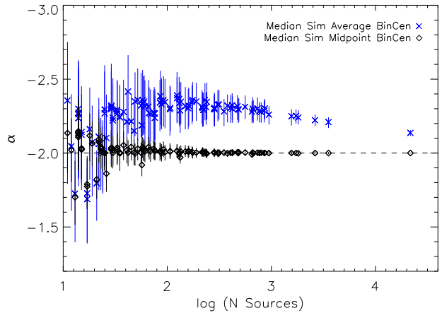
Figure 7. The plot of simulated LF slopes for two bin center definitions, where blue asterisks represent the average of logarithmic luminosities in each bin and the black diamonds represent the midpoint of the logarithmic luminosities in each bin. The average bin center definition results in a bias towards steeper LF slopes compared to the input -2 LF slope, while the midpoint bin center definitions recover the input -2 LF slope. We use the midpoint bin center definition to construct our LFs.
