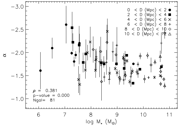
Figure 12. A plot of the LF slope ( \alpha ) versus stellar mass ( M_* ) similar to that of Figure 10. We find a weak trend between these two quantities similar to that found for M_B .
