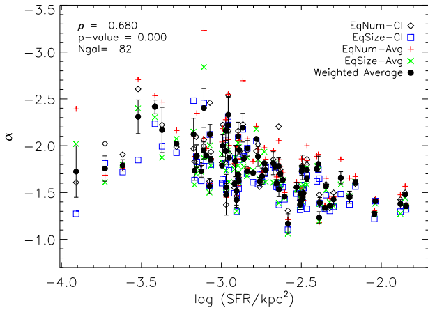
Figure 17. A plot of the LF slope ( \alpha ) versus \Sigma_{\text{SFR}} where we have combined 2 photometry methods and 2 LF binning methods to produce 4 combinations of the LF slope. This graphically shows the systematics of our methods. We find a strong trend between these \alpha and \Sigma_{\text{SFR}} when using a weighted average LF slope for the 4 combinations of photometry and binning methods.
