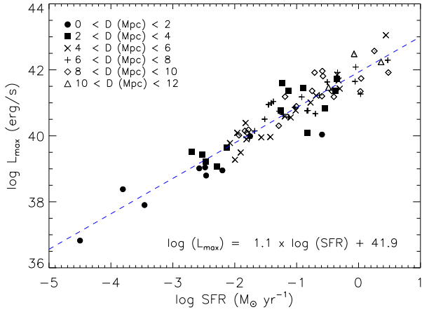
Figure 24. A plot of the luminosity of the brightest star-forming region ( L_{\max} ) and SFR. We find a tight correlation with a correlation coefficient ( \rho ) of 0.904. Since the global SFR of a galaxy scales with the total number of sources, this tight trend indicates that a “size-of-sample” effect is present in our sample. However, both the real and simulated LFs of galaxies with low number statistics show random scatter both above and below the canonical -2 LF slope suggesting that the “size-of-sample” effect is not responsible for the trends between LF slope and galaxy properties.
