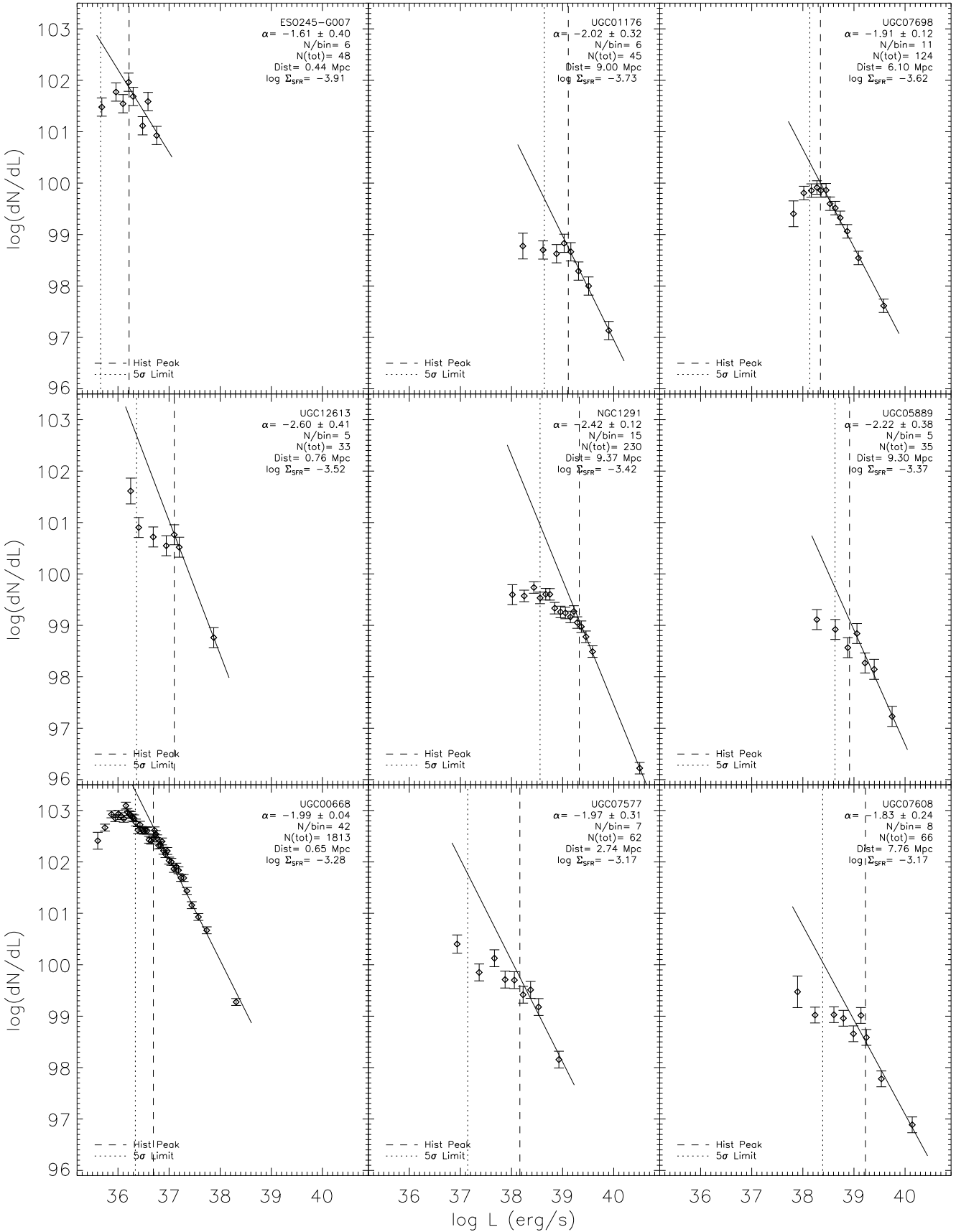
Figure A1. Figures A1- A10 show the LFs for all 82 galaxies in our final sample, where the panels have been sorted by \Sigma_{\text{SFR}} . The y-axes for all LFs in all figures have been normalized to the same arbitrary number to facilitate comparisons of all luminosity functions.
