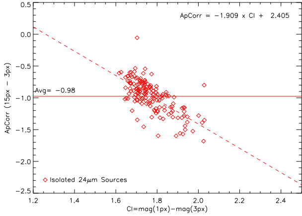
Figure 4. The plot of aperture correction versus concentration index for isolated 24\mu\text{m} sources. The relationship shows that more extended objects require a larger aperture correction.
