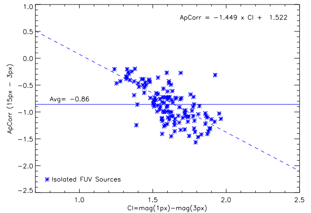
Figure 3. The plot of aperture correction versus concentration index for isolated FUV sources. The aperture correction is defined as the magnitude difference at 15 and 3 pixel radii (the photometry aperture) and the concentration index is defined as the magnitude difference at 1 pixels and 3 pixels. Concentration index is a measure of a source's radial profile extent and the relationship shows that more extended objects require a larger aperture correction.
