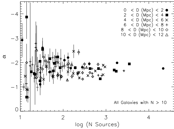
Figure 18. A plot of the LF slope ( \alpha ) versus number of sources similar to that of Figure 10. We find increased scatter towards lower numbers of sources, and decreased scatter towards higher numbers of sources. The average slope of all LFs is -1.76 \pm 0.30 (median = -1.75 ).
