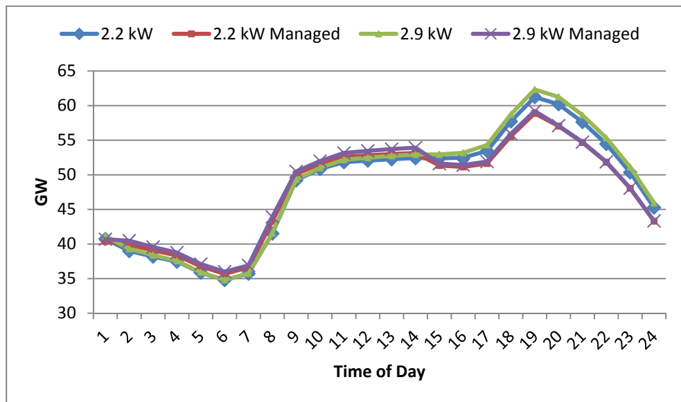
Figure 22: Effects of Charging Power on the Overall Electricity Demand (for BAU Scenario for EV uptake)
