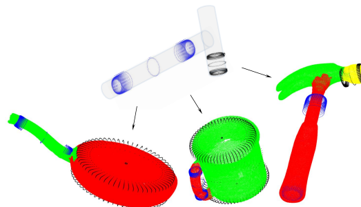
Fig. 1. Typical fits by our system for projecting an idealised model of a hammer (source) onto a hammer, mug, and frying pan (target objects). Each model part is projected into a segment of the point cloud. The task model defines how various distortions of parts, and the relationship among parts, are to be penalised.
