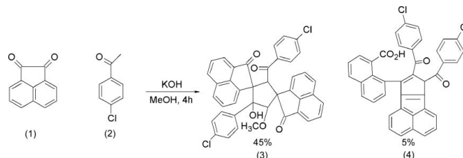
Figure 1 Reaction scheme showing the synthesis of the title compound (4).
