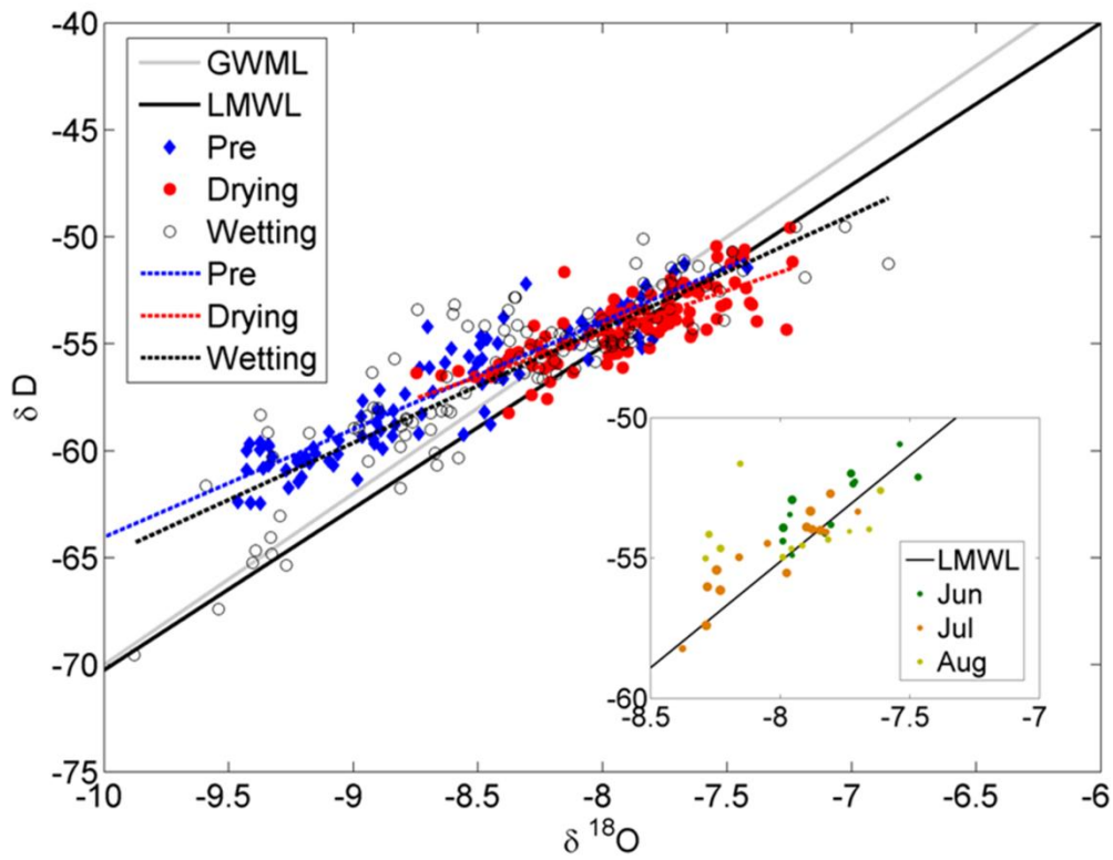
Figure 10: Stream water stable isotopes on the global and local meteoric water line, for the three different hydroclimatic periods (main figure) and for three months in summer, during which no precipitation was observed with symbol size reflecting the relative potential evapotranspiration of that day (lower right inset).
