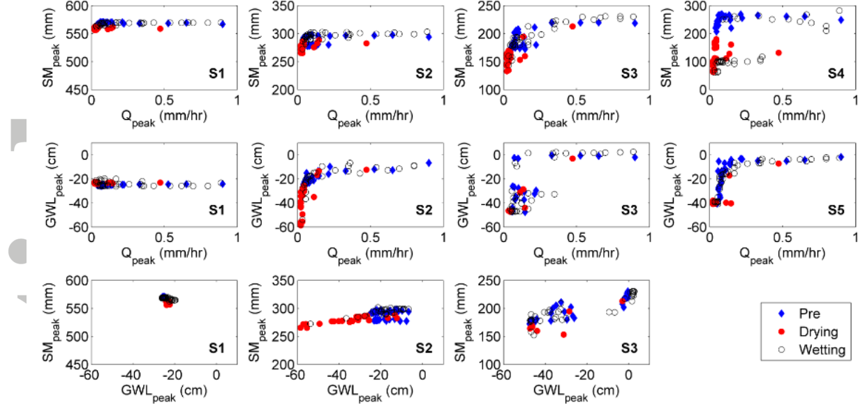
Figure 6: Event Magnitude Characteristics for the ‘pre-drying’, ‘drying’ and ‘wetting’ periods, respectively. The top and middle rows show the peak response in soil moisture and groundwater, respectively, versus the peak in discharge and the bottom row the peak response in soil moisture versus peak response in ground water level. Note the difference in scale for soil moisture at S4, compared to S1-S3, and the different absolute range for S1. The last plots of the top and middle row are from different sites (S4 and S5 respectively), due to lack of data availability.
