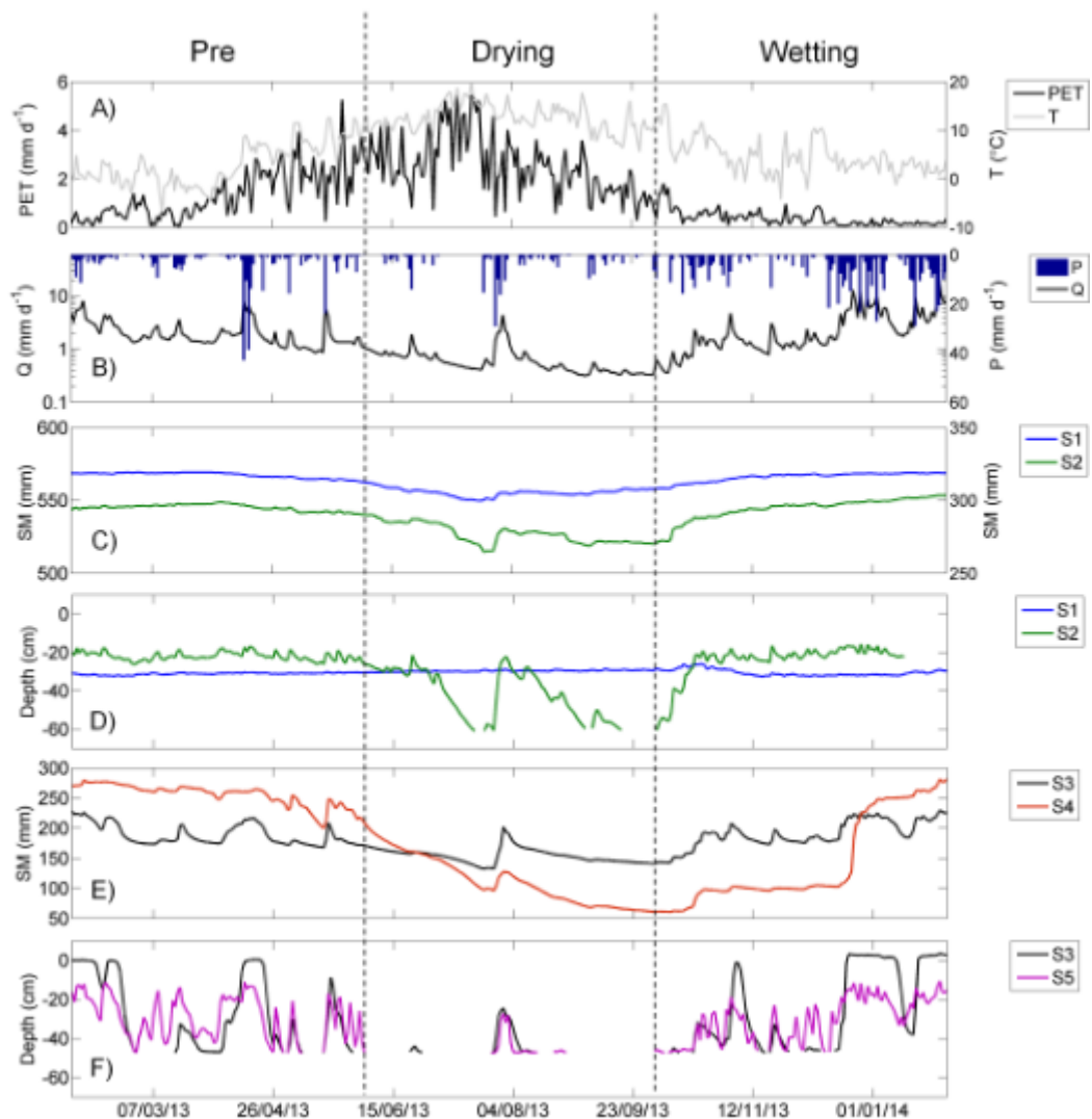
Figure 3: Temporal dynamics (01/02/2013 – 31/01/2014) in daily (a) Air Temperature and Potential Evapotranspiration, (b) Precipitation and Discharge for the Bruntlan Burn and (c) Soil Moisture, and (d) Shallow Groundwater Levels for Histosols (S1 and S2) and (e and f) Podzols (S3 and S4,S5), respectively. Distinct catchment drying and re-wetting occurred in the periods 01/06 – 30/09 and 01/10 – 31/01 respectively, as indicated by the dotted lines.
