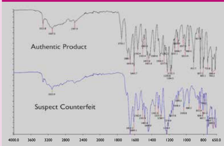
Figure 2: FT-IR spectra shows that a suspect headache powder does not match an authentic product
