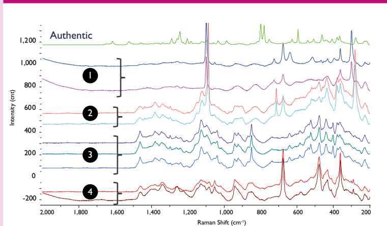
Figure 1: Comparison of mean Raman spectra for an authentic tablet and 4 counterfeit tablets
