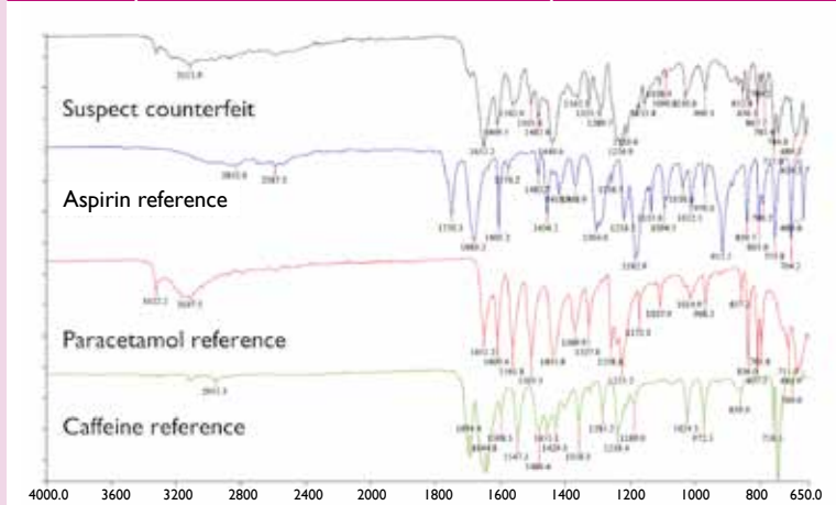
Figure 3: FT-IR comparison shows that the suspect powder contains paracetamol and caffeine, but no aspirin
