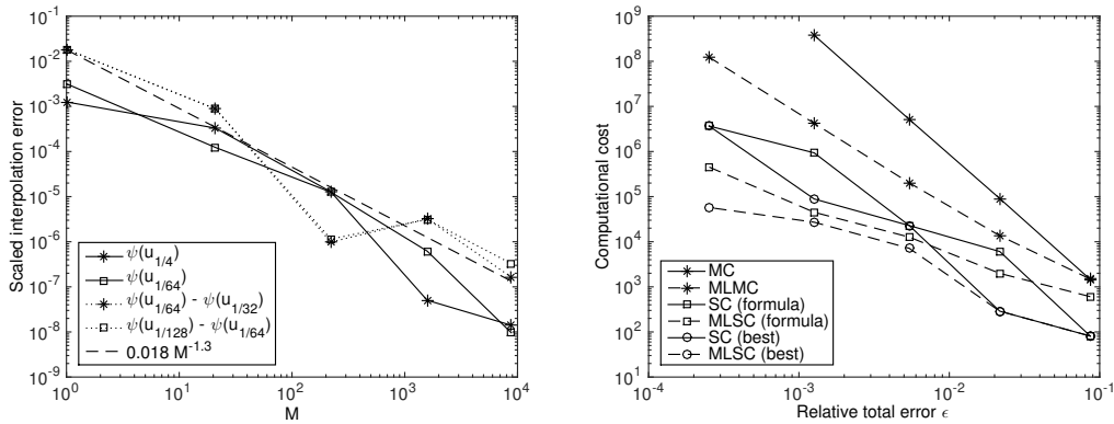
Figure 6.3. D = (0, 1)^2 , N = 10 . Left: \mathbb{E}[\mathcal{I}_{M_5} \psi(u_h) - \mathcal{I}_{M_k} \psi(u_h)]/h_0^2 and [\mathcal{I}_{M_5}(\psi(u_h) - \psi(u_{2h})) - \mathcal{I}_{M_k}(\psi(u_h) - \psi(u_{2h}))]/h^2 versus M_k , for various h . Right: computational cost versus relative error \varepsilon .
