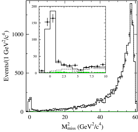
FIG. 7 (color online). The M_{\text{miss}}^2 distribution for data (points with error bars) with 2.8 < M_{K^+K^-} < 3.0 \text{GeV}/c^2 selected with all the criteria described in Sec. III except for the requirement |M_{\text{miss}}^2| < 1 \text{GeV}^2/c^4 . The solid histogram is a sum of signal and background distributions obtained from MC simulation. The dashed histogram shows the distribution for two-photon events, and the shaded (almost invisible) histogram shows the small contribution of all other background processes. The inset shows an enlarged view of the region -2 < M_{\text{miss}}^2 < 10 \text{GeV}^2/c^4 . Above 10 \text{GeV}^2/c^4 the solid and dashed histograms are indistinguishable.
