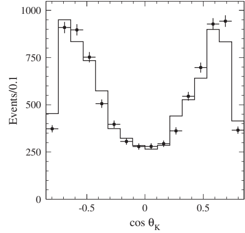
FIG. 8. The \cos \theta_K distribution for data (points with error bars) and reweighted simulated events (histogram) with M_{\text{miss}}^2 > 20 \text{GeV}^2/c^4 from the K^+K^- mass range 2.8–3.0 \text{GeV}/c^2 .
