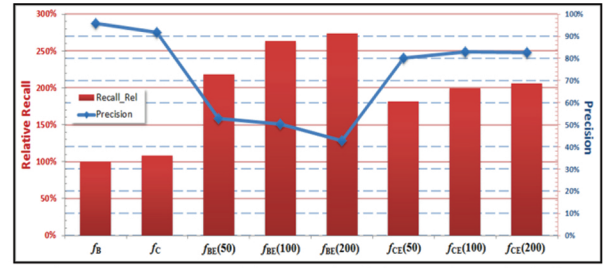
Figure 2 Average precision (on the right Y-axis) and relative recall (on the left Y-axis) achieved for tweets tracking using different approaches, tested on 3 broad topics over 4 test days.
