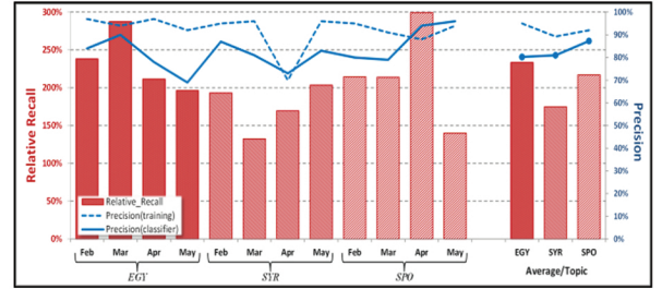
Figure 3. Topic tracking performance across different topics and over time for f_{CE}(200)
