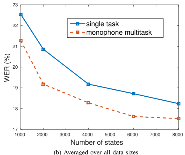
Fig. 4. Comparing standard DNNs with the use of monophones as a secondary task with varying number of tied states.
