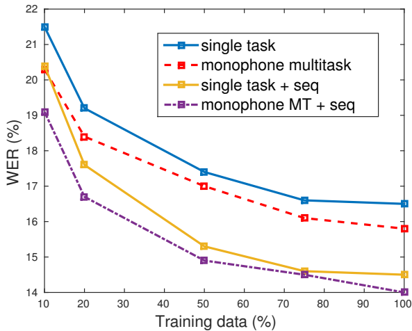
(a) Varying training data, 8000 states
