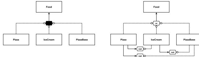
Fig. 2: Example of a disjoint concept hierarchy represented in Graphol with (left-hand side figure) and without (right-hand side figure) the disjoint union node.
