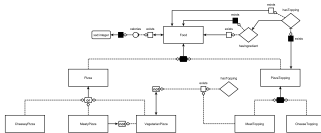
Fig. 4: Graphol ontology example: an excerpt of the Pizza ontology.
