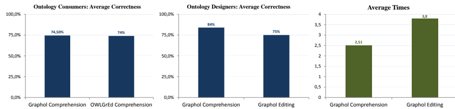
Fig. 5: Average results for percentage of correct answers and for overall times.
