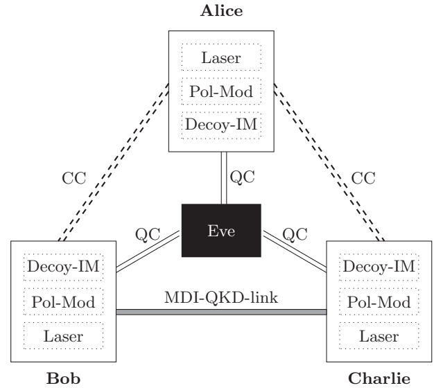
FIG. 1. Schematic diagram of a setup for MDI-QDS. Alice, Bob, and Charlie prepare quantum signals in different BB84 polarization states, using a polarization modulator (Pol-Mod). In addition, they generate decoy states with an intensity modulator (Decoy-IM). The signals are then sent to an untrusted party Eve, who acts like a relay and is supposed to perform a Bell state measurement, which projects the incoming signals into a Bell state. The channels between Alice-Eve, Bob-Eve, and Charlie-Eve are quantum channels (QC). Eve performs the measurement separately for the pairs Alice-Bob and Alice-Charlie. Bob and Charlie share a MDI-QKD link (gray channel), which can be used to transmit classical messages in full secrecy. The pairs Alice-Bob and Alice-Charlie have pairwise authenticated classical channels (CC) indicated as dashed lines, through which they can communicate their basis settings for the different key positions.
