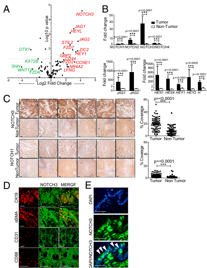
Fig. 1. Notch3 is differentially activated in human CC. (A) Volcano plot of rPCR Notch array in human CC and patient-matched liver ( n = 5 , n = 5 ). Gray line represents P value of 0.05. Red labels, up-regulation at least fourfold; green, down-regulation at least fourfold. (B) Notch expression in human CC ( n = 48 ) and healthy liver ( n = 42 ) (RT-PCR). Medians compared with Mann-Whitney U test. (C) Tissue microarray human CC ( n = 77 ) and noncancerous liver ( n = 47 ). Representative Notch1 and Notch3 immunostaining (positive and isotype controls; Fig. S1 B and C). Filled arrowheads, Notch3 + ductules and vascular smooth muscle in healthy liver. Pixel analysis of CC and controls compared with Mann-Whitney U test. (D) Dual fluorescence of Notch3 (green) in human CC with \alpha SMA, CD31 + , or CD68 + (red) (Scale bar, 100 \mu m.) (E) N3-ICD (green) in human CC (white filled arrowheads). (Scale bar, 50 \mu m.) Data are means \pm SEM. * P \leq 0.05 , ** P \leq 0.01 , *** P \leq 0.001 .
