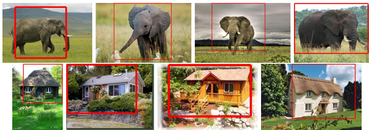
Fig. 8: Highest scoring “objectness” regions (in red) when images downloaded from Bing/Google are passed into an RPN. Top row: ‘elephant’, Bottom row: ‘cottage’. Notice that the regions manage to contain the object, with quite a tight bound.
