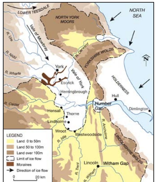
Figure 1. Regional ice limits of the Last Glacial Maximum, with ice flow directions and the York and Escrick moraines. (After Clark et al. , 2004.)
