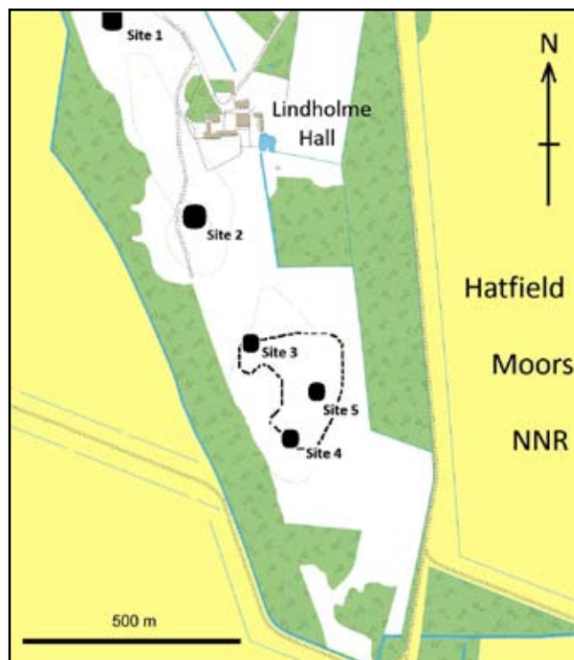
Figure 3. Locations of exposures on Lindholme.
