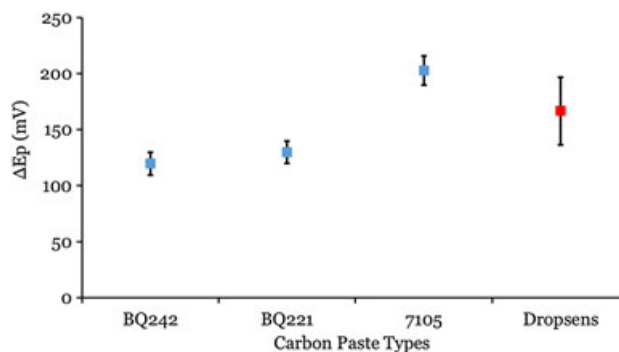
Figure 4. Graphical representation of the electrochemical characterisation via cyclic voltammetry of different DuPont carbon pastes and Dropsens SPCE. Cyclic voltammetry's were recorded at a scan rate of 50 \text{ mV s}^{-1} in the presence of the redox pair \text{Fe}(\text{CN})_6^{3-/4-} (10 mM in phosphate buffer), and the average peak separation between the observed oxidation and reduction potentials ( \Delta E_p ) were recorded as a function of the electrode surface. Error bars represent standard deviation ( n = 10 ).
