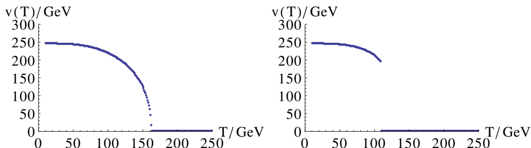
Figure 1. Examples of the order parameter dependence on temperature for the effective model. On the left, a second order transition ( T_c \simeq 160 GeV). On the right a first order transition ( T_c \simeq 105 GeV).
