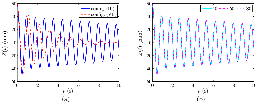
FIGURE 3. Time series of vertical model motions Z(t) for: a) configurations (III) and (VII), illustrating the dramatically different decay rates obtainable with simple tuning; b) three different release heights for configuration (III), scaled to initial release height of 60mm.
