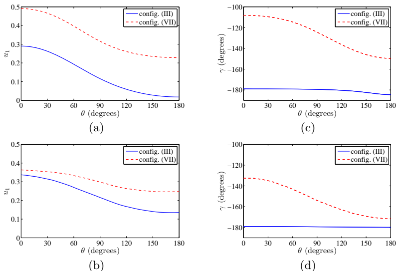
FIGURE 5. Predicted magnitude ((a) and (b)) and phase ((c) and (d)) of the vertical fluid velocity on the cylinder sides, relative to the body velocity, for configurations (III) and (VII). (a) and (c) show these parameters at the top of the cylinders, (b) and (d) at the bottom (note that the drafts of these configurations are not equal). Due to symmetry only half of each cylinder need be shown. 0^\circ is the point on the cylinder closest to the centre of the ring.
