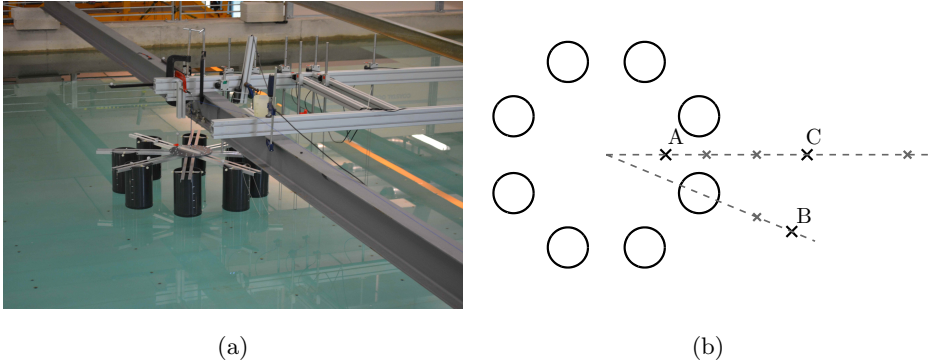
FIGURE 1. a) A photograph of the experimental set-up, with the wave gauges to the right of the picture. b) Layout of the 7 wave gauges used, relative to the cylinders at radius 5a . Only those gauges referred to in this paper are labelled. Gauges were not moved between tests - gauge A is at radius 2.96a from the centre of the ring, and gauges B and C at 10a .
