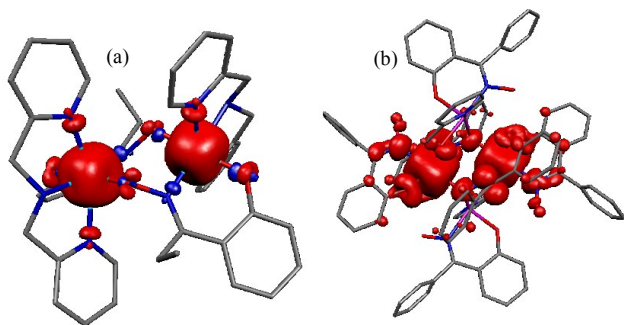
Figure 6. Computed spin density HS plot for complex 1 (a) and complex 6 (b).
