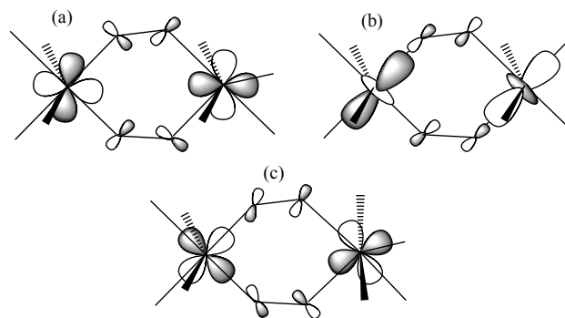
Figure 5. Schematic representation of the (a) d_{xy} - d_{xy} overlap in complexes 1-5 , (b) d_z^2 - d_z^2 overlap in complex 6 , (c) cross-interaction between d_{x^2-y^2} and d_{xz} in complexes 1-6 .
