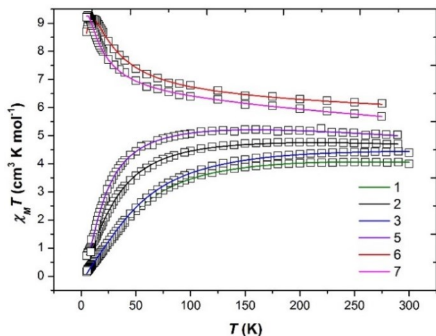
Figure 4. Plot of the \chi_M T product versus T for complexes 1-3 , 5-7 . The solid lines are a fit of the experimental data to isotropic spin-Hamiltonian (1). See text for details of the best fit parameters. Green = 1 , black = 2 , blue = 3 , purple = 5 , red = 6 and pink = 7 .
