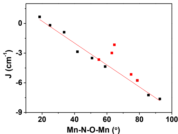
Figure 7. Magneto-structural correlations developed by varying the Mn-N-O-Mn dihedral angle in 1 . The red squares are experimental J values obtained for complexes 1-6 .
