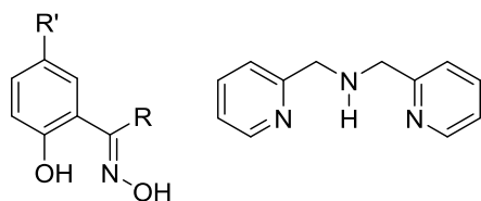
Figure 2. Left: generic structure of a phenolic oxime. saoH 2 , R = R' = H; Me-saoH 2 , R = Me, R' = H; Et-saoH 2 , R = Et, R' = H; Ph-saoH 2 , R = Ph, R' = H; Me 2 -saoH 2 , R = R' = Me. Right: di-(2-picoyl)-amine, dpa.
