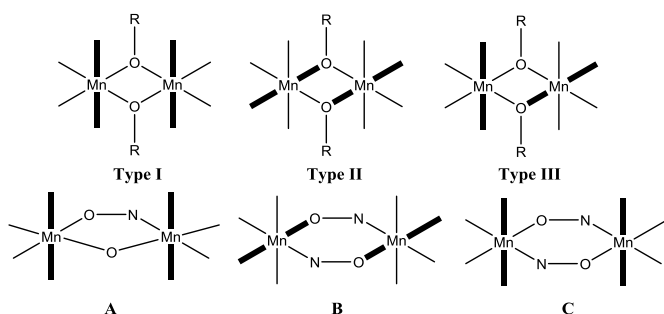
Figure 1. Top: alkoxide bridged dimers [\text{Mn}^{\text{III}}(\text{OR})_2] with Type I–III structures differing in the relative orientations of the Jahn-Teller axes, which are highlighted in bold. Bottom: oxime/oxo dimers [\text{Mn}^{\text{III}}_2(\text{O})(\text{NO})] ( A ), and the double oxime bridged dimers [\text{Mn}^{\text{III}}(\text{NO})_2] in which the Jahn-Teller axes lie in the bridging plane ( B ), and perpendicular to the bridging plane ( C ).
