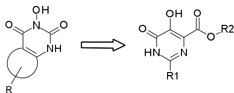
Figure 2. Scaffold hop to hydroxypyrimidinone motif 11
