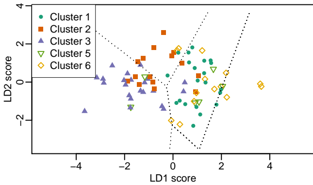
(a) Scores for the first two discriminant functions. LDA decision boundaries are shown with dotted lines.
