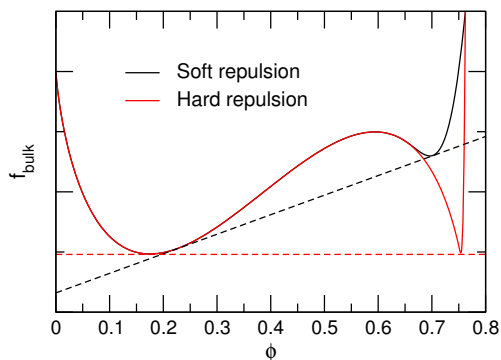
Fig. 6 Bulk free energy f_{\text{bulk}} = f_0 + f_{\text{rep}} as given by Eqs. (10) and (17), obtained using v = v_0(1 - 1.3\phi) , and the parameter values \{k_{\text{rep}}, \phi_l\} = \{10^3, 0.64\} (“Soft repulsion”) and \{10^7, 0.75\} (“Hard repulsion”), respectively. The dashed lines denote approximate common-tangent constructions, yielding the coexistence densities \{\phi_g, \phi_l\} = \{0.23, 0.70\} and \{0.18, 0.75\} for the “soft” and “hard” curves, respectively. Terms linear in \phi are irrelevant for the common-tangent construction and have been subtracted for clarity.
