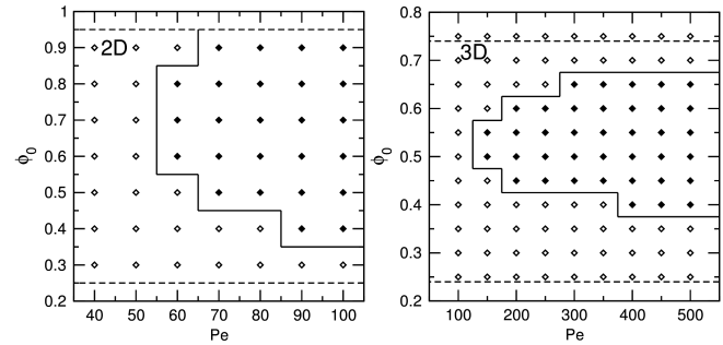
Fig. 1 Phase diagrams in the Pe - \phi_0 plane as determined from ABP simulations of systems with size L_{\text{box}} = 150\sigma (2D, left panel) and L_{\text{box}} = 30\sigma (3D, right panel). Open symbols denote state points with a homogeneous density, and filled symbols denote points with phase-separated steady states. Solid lines show the approximate spinodals, while the dashed lines denote the approximate high- Pe asymptotes for the binodal densities, determined for Pe = 100 (2D) and Pe = 300 (3D). The locations of the spinodals were determined both by visual inspection and by examining the growth in the characteristic length-scale L(t) , as further described in Section 4.3. The lower binodal densities (0.25 and 0.24 in 2 and 3 dimensions, respectively) were determined using larger systems ( L_{\text{box}} = 1000\sigma and L_{\text{box}} = 100\sigma in 2D and 3D, respectively) by starting from fully phase-separated states, while the upper boundaries were determined by approximate extrapolation to the case of vanishing volume of the dilute phase.
