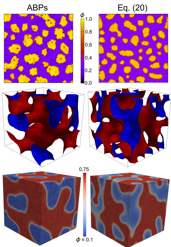
Fig. 4 Snapshots obtained from an ABP simulation (left) and by numerically solving Eq. (20) (right), both at average packing fraction \phi_0 = 0.5 . Snapshots are taken at equal times of t = 500\tau_r ( t = 100\tau_r ) in 2D (3D). The continuum and ABP systems are of approximately equal size L = 60\lambda (2D, top panel) and L \approx 21\lambda (3D, center and bottom panels). The bottom panel shows 2D projections of the 3D density field, obtained from the same configurations as the isosurfaces in the center panel.
