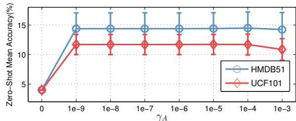
Fig. 12 Zero-shot mean accuracy v.s. ridge regression parameter
