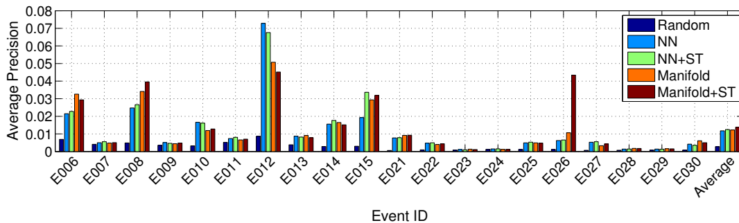
Fig. 3 Zero-shot performance on TRECVID MED 2013 measured in mean average precision (mAP).
