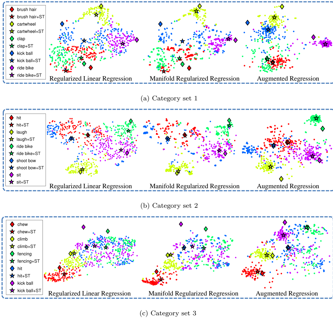
Fig. 4 A qualitative t-SNE illustration of ZSL with semantic space representation for random testing class subsets (a), (b) and (c). Variants: ridge regression, manifold regression and data augmented manifold regression. Dots indicate instances, color categories, and star/diamond show category prototypes with/without self-training.
