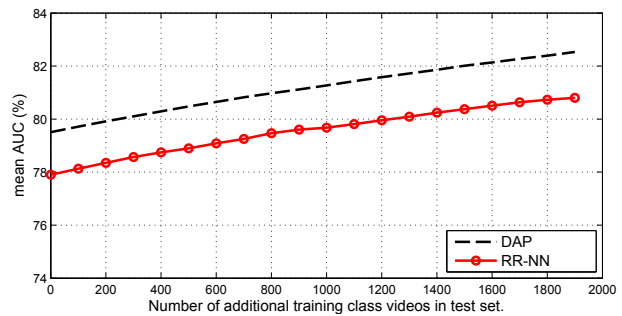
Fig. 8 Injecting training/known class samples to testing set.
