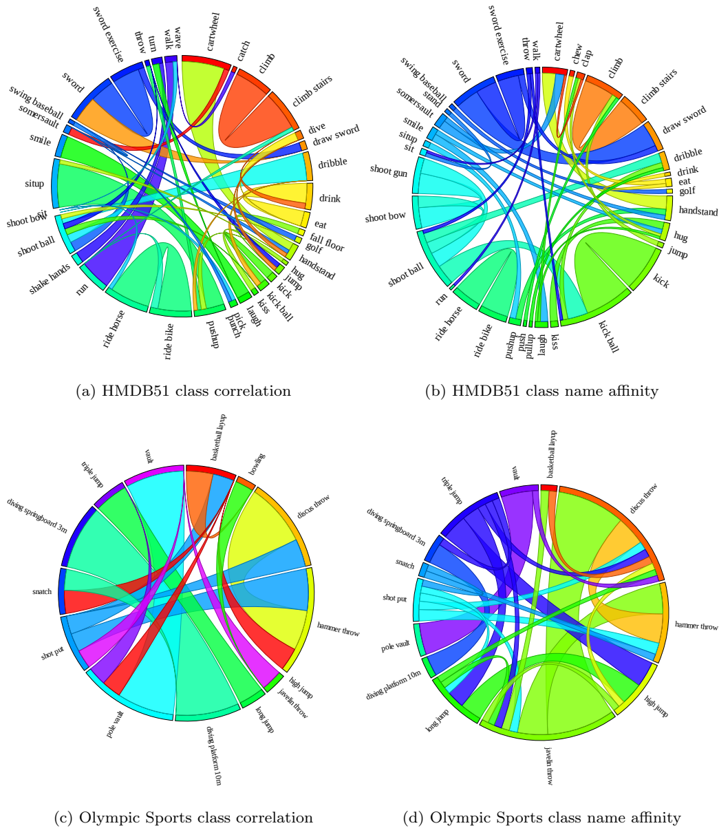
Fig. 5 Chord Diagram to illustrate the category correlation discovered from zero-shot recognition experiments. (a) and (c) illustrate the correlation discovered from 50 random split zero-shot experiments; (b) and (d) illustrate the class name affinity in word-vector embedding space measured as cosine similarity.
