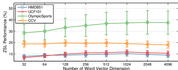
Fig. 11 Zero-shot performance v.s. dimension of word-vector.
