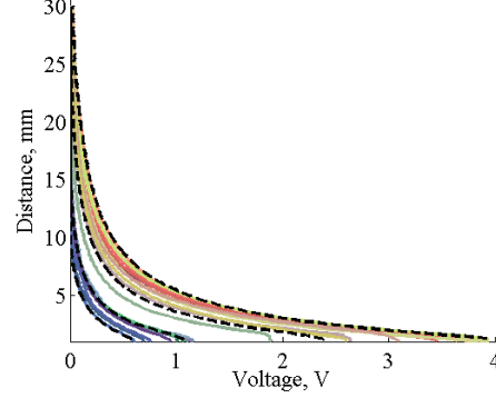
Fig. 8: Obtained color code mapped to voltage responses from the proximity sensor. Black lines show calibration curves, and colored lines correspond to voltage responses from the proximity sensor, the color of the line reflects RGB color value from the camera.
