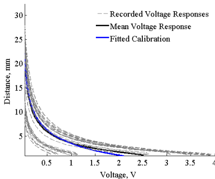
Fig. 6: Calibration curve obtained using average sensor response.
