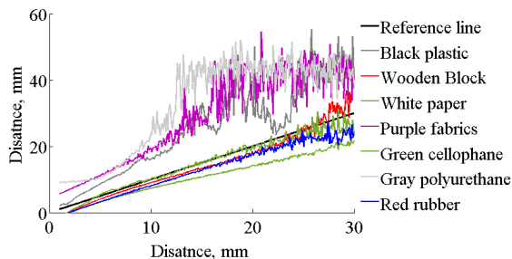
Fig. 10: The results of distance estimation without the use of calibration algorithm and without an external camera relatively the linear reference line ( x = y ).
