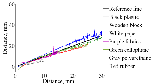
Fig. 9: The results of distance estimation using calibration algorithm relatively the linear reference line ( x = y ).
