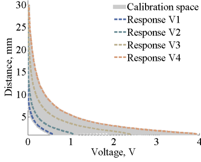
Fig. 7: Selected voltage responses used for calibration in the calibration space.
