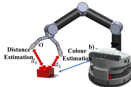
Fig. 1: System working principle: FESTO mobile robotic platform (a) makes use of a vision system (b) to detect the color of an object to be grasped with its robotic Metha-Hand(c). The hand is endowed with a fiber optic proximity sensor to evaluate the distance between the hand and the object, the color information collected by the camera is used to adjust in real time the calibration curve of the sensor.
