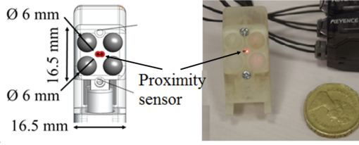
Fig. 2: Design and prototype of the fingertip with integrated proximity and four tactile sensors.
