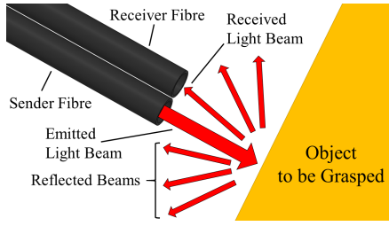
Fig. 4: Working principle of fiber optical proximity sensor.
