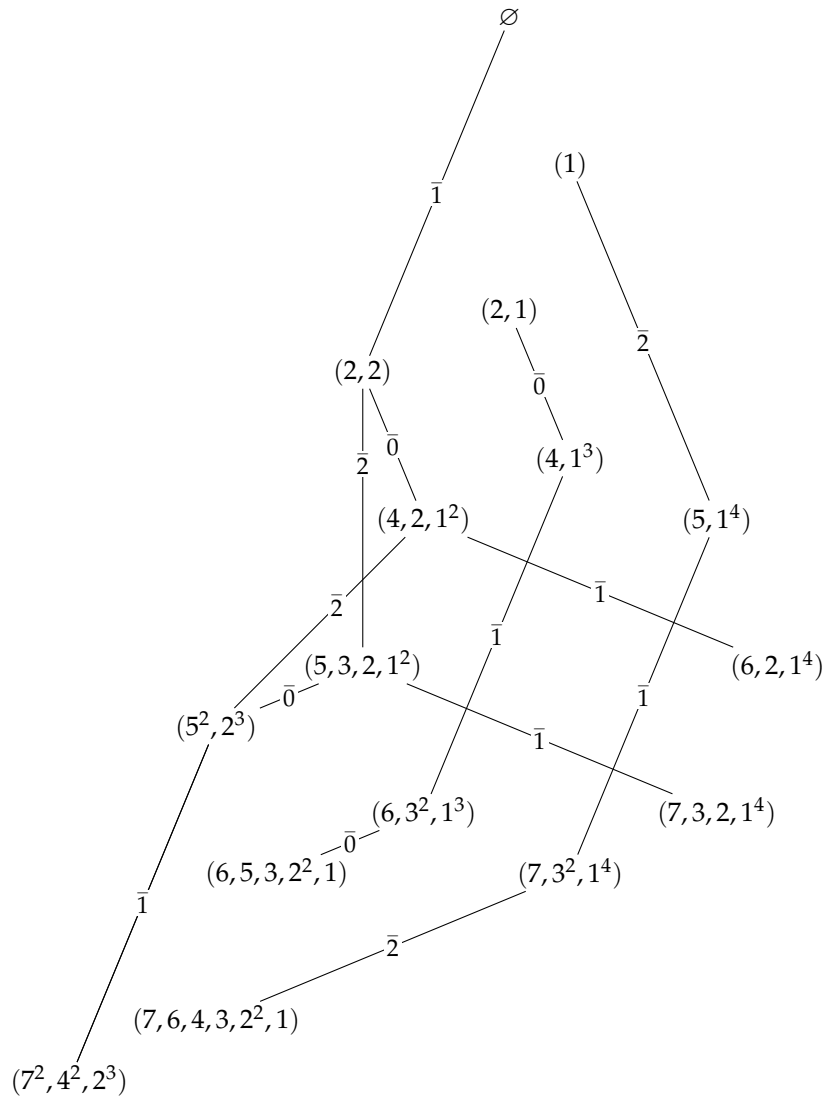
Figure 7: The level 2 action of \tilde{\mathcal{H}}_5 on \mathcal{D}_5^{(4)}
