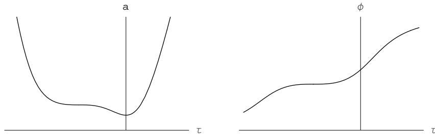
FIG. 5: The time evolution of a and \phi for n = -2 , \omega = -10 , c_3 = 10 and \gamma = 4/3 .
