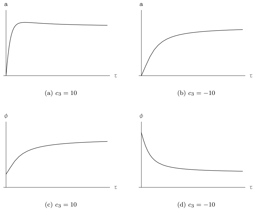
FIG. 2: The time evolution of a and \phi for n = 2 , \omega = -10 and \gamma = 4/3 .
