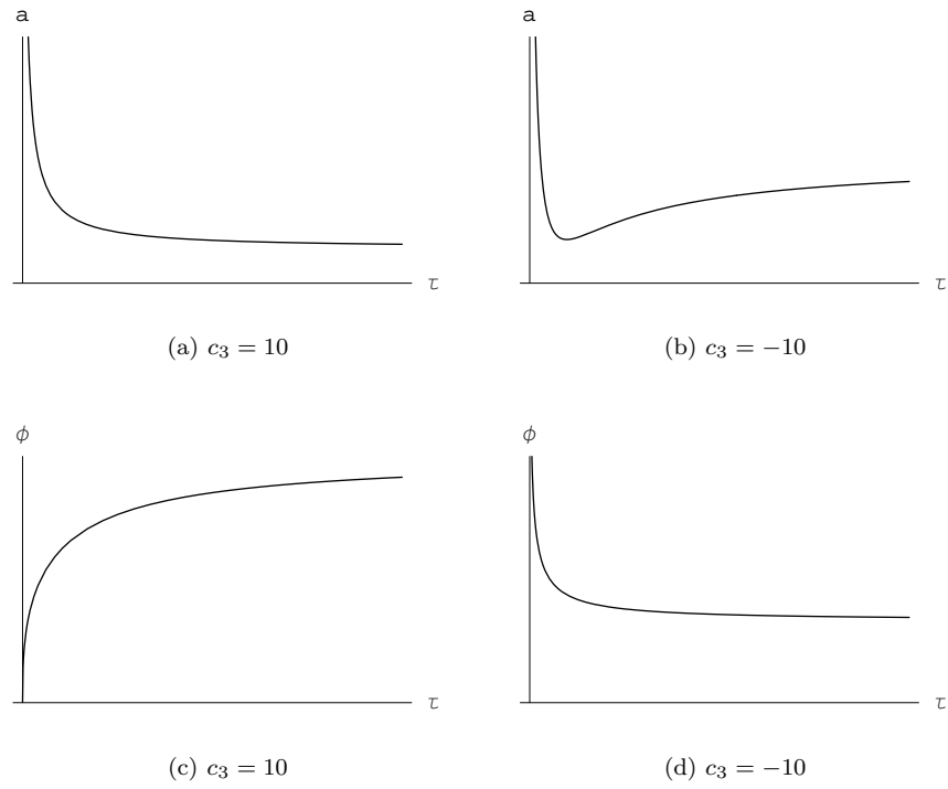
FIG. 1: The time evolution of a and \phi for n = 2 , \omega = 10 and \gamma = 4/3 .
