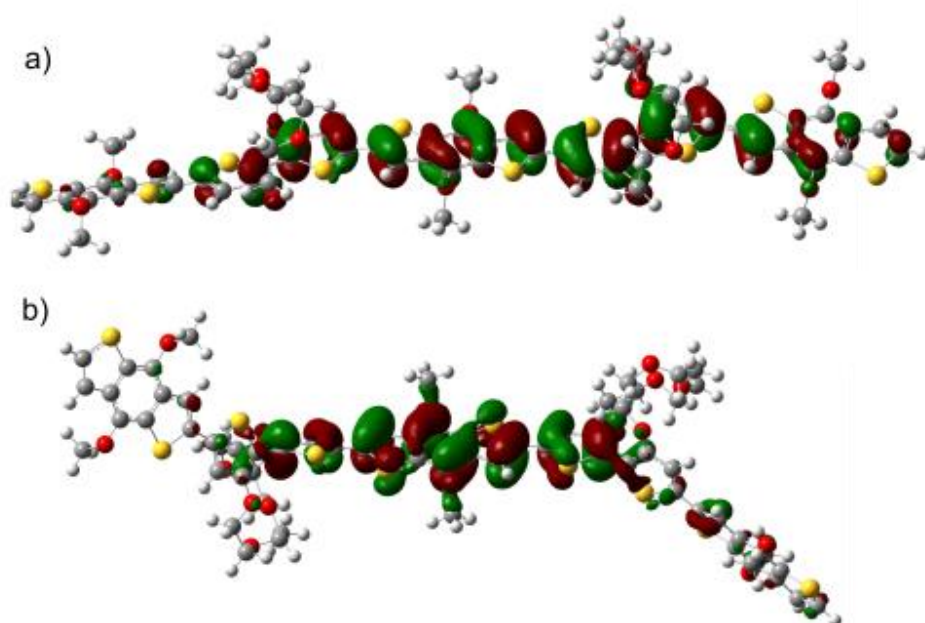
Figure 6: HOMO of a planar and twisted molecule with three BDT and two T2 units.
