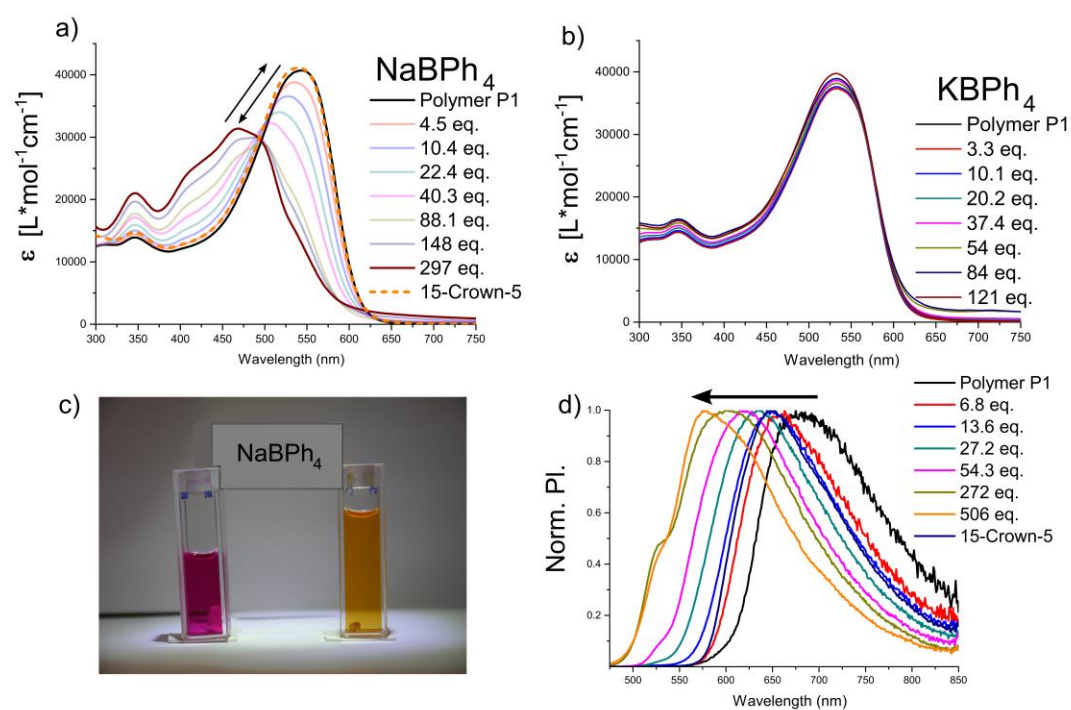
Figure 5: (Figure changed, \text{NaBPh}_4 was missing) Titration experiments of P1 and \text{MBPh}_4 ( M = \text{Na}, \text{K} ) in THF, a) addition of \text{NaBPh}_4 and 15-Crown-5 b) addition of \text{KBPh}_4 , c) color change after addition of 300 eq. \text{NaBPh}_4 . d) PL shift with \text{NaBPh}_4 .
