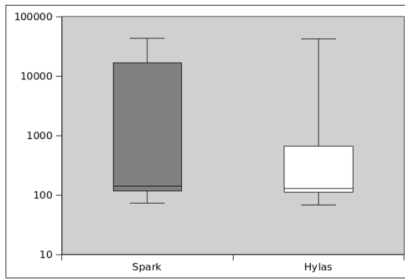
Figure 2: Boxplot for Spark vs Hylas execution times given in seconds
