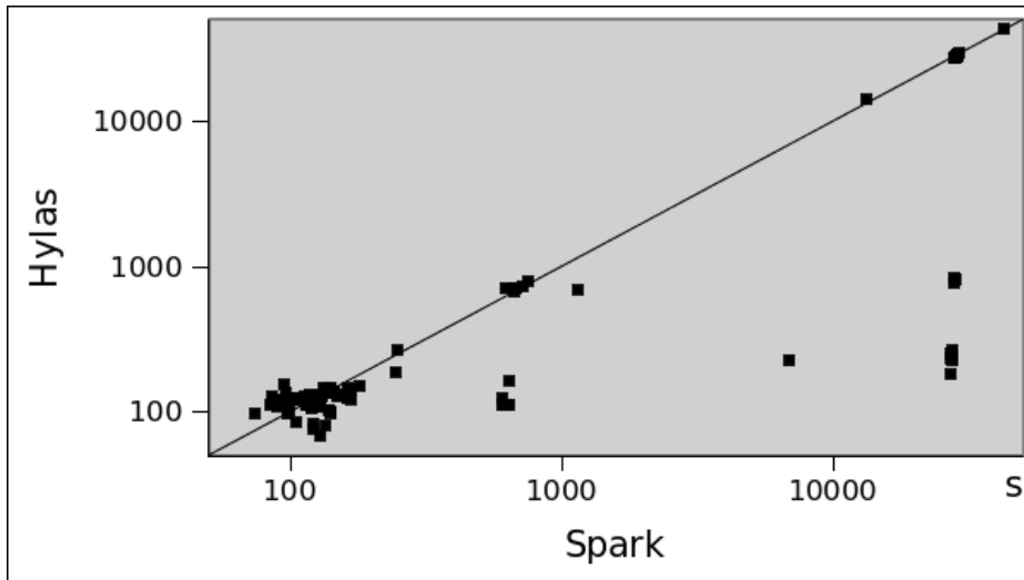
Figure 1: Spark vs Hylas execution times (seconds) for all queries
